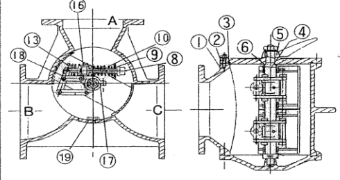
Fig-4* 200A/250A
