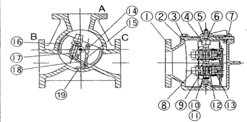
Fig-4* 200A/250A
