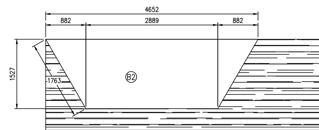
BOTTOM PLATE THICKNESS 6mm 6000x2000 2 PIECES
