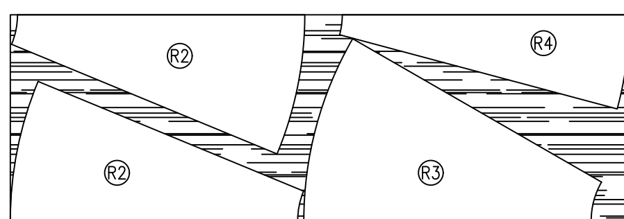
PL.6000x2000 THICKNESS 5mm 1 PIECE
