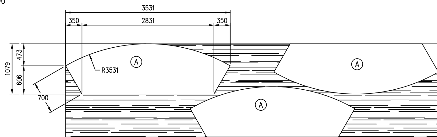
ANNULAR BOTTOM PLATE THICKNESS 6mm 8000x2000 2 PIECES
