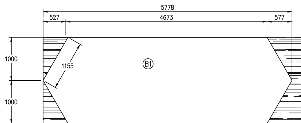
BOTTOM PLATE THICKNESS 6mm 6000x2000 1 PIECE
