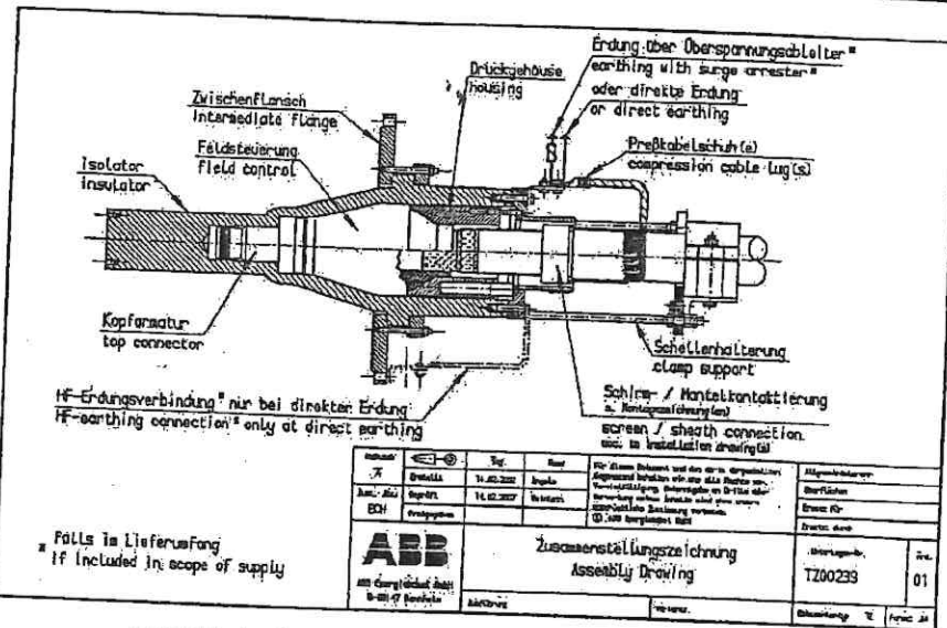
assembly drawing of EHSVS 245-300, type E / EHSVS 362-550, type F
