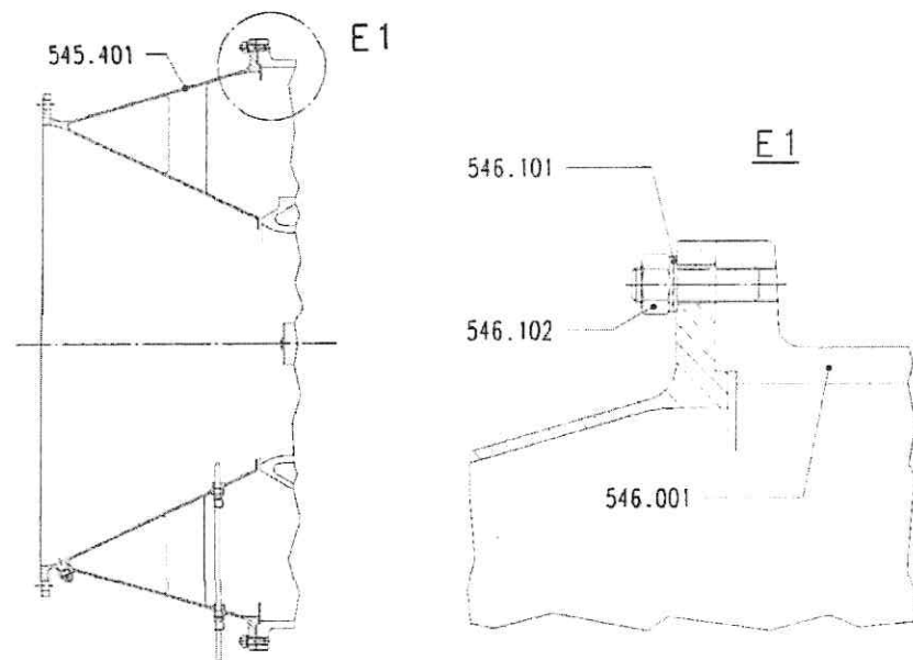
Figure 1: Removing and refitting the air intake casing
