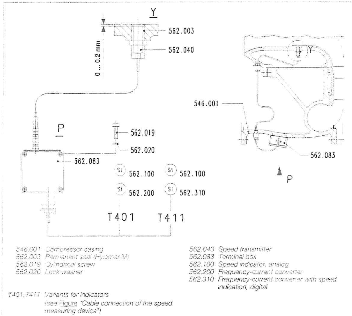
Figure 2: Speed measuring device
