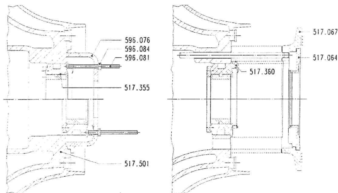
Figure 1: Removing and refitting the plain bearing
