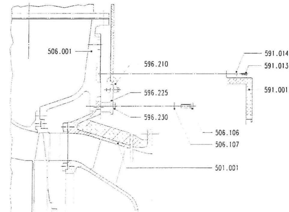
Figure 1: Removing and refitting the gas admission casing
