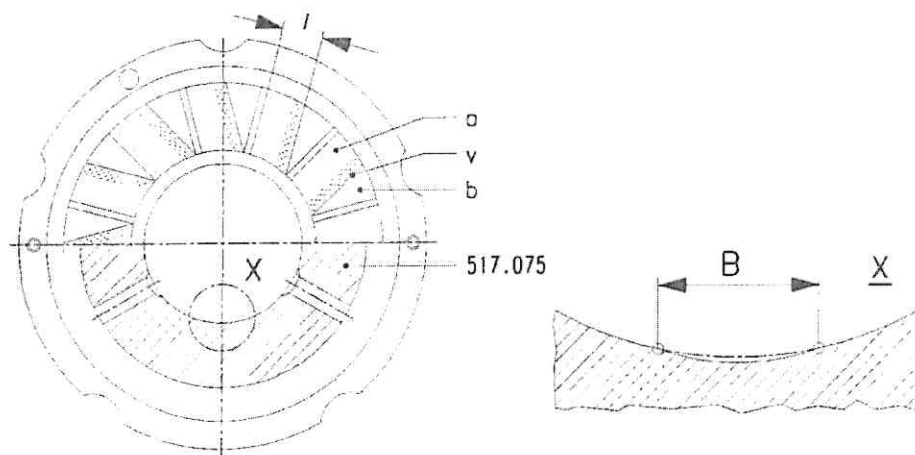
Figure 1: Checking the locating bearing (517.075).
