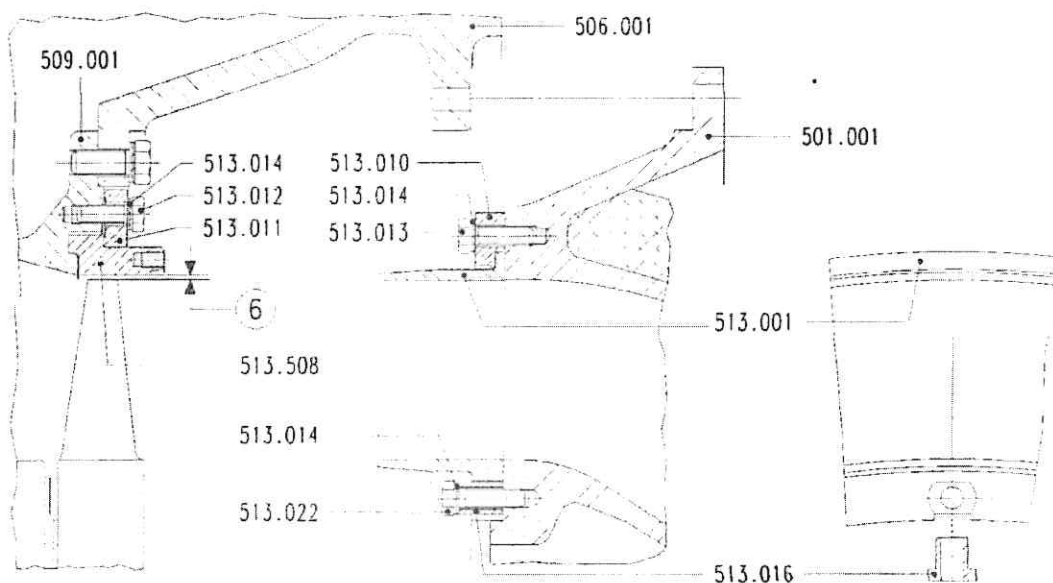
Figure 1: Removing and refitting the nozzle ring and shroud ring
