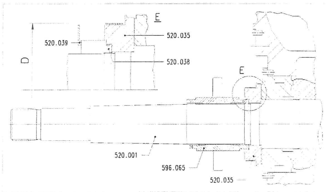
Figure 1: Removing, checking and refitting the locating ring
