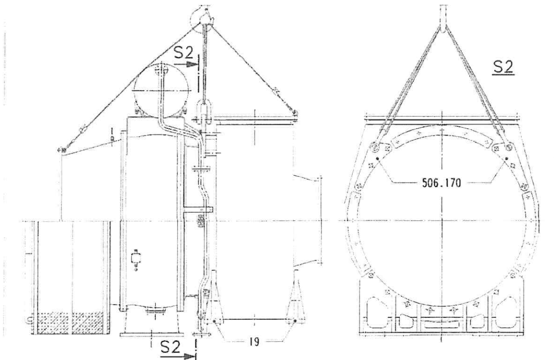
Figure 2: Removing and refitting the complete turbocharger NA57/T9
