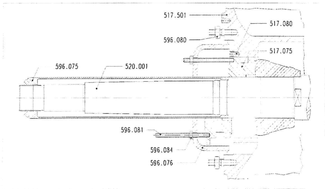
Figure 1: Removing and refitting the locating bearing
