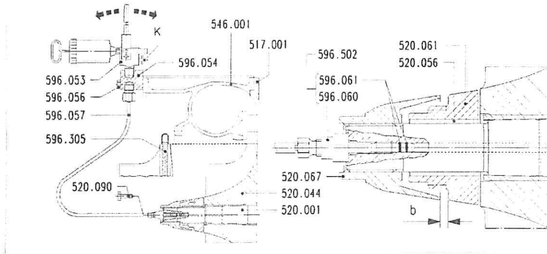
Figure 1: Removing the compressor wheel
