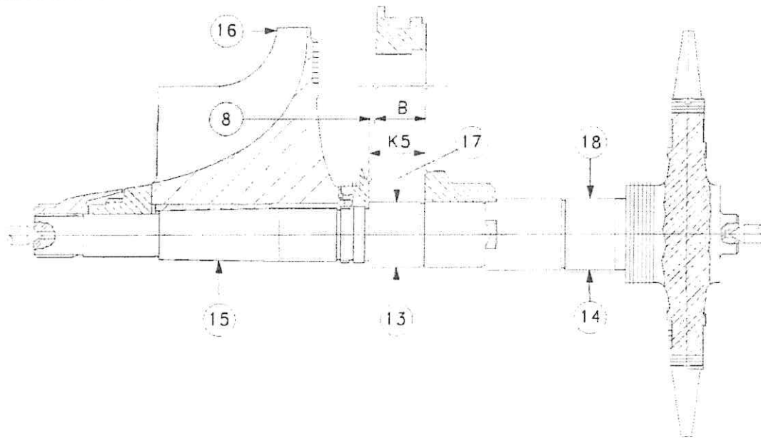
Figure 2: Measurement of the axial clearance (8), measuring points, radial and axial runout
