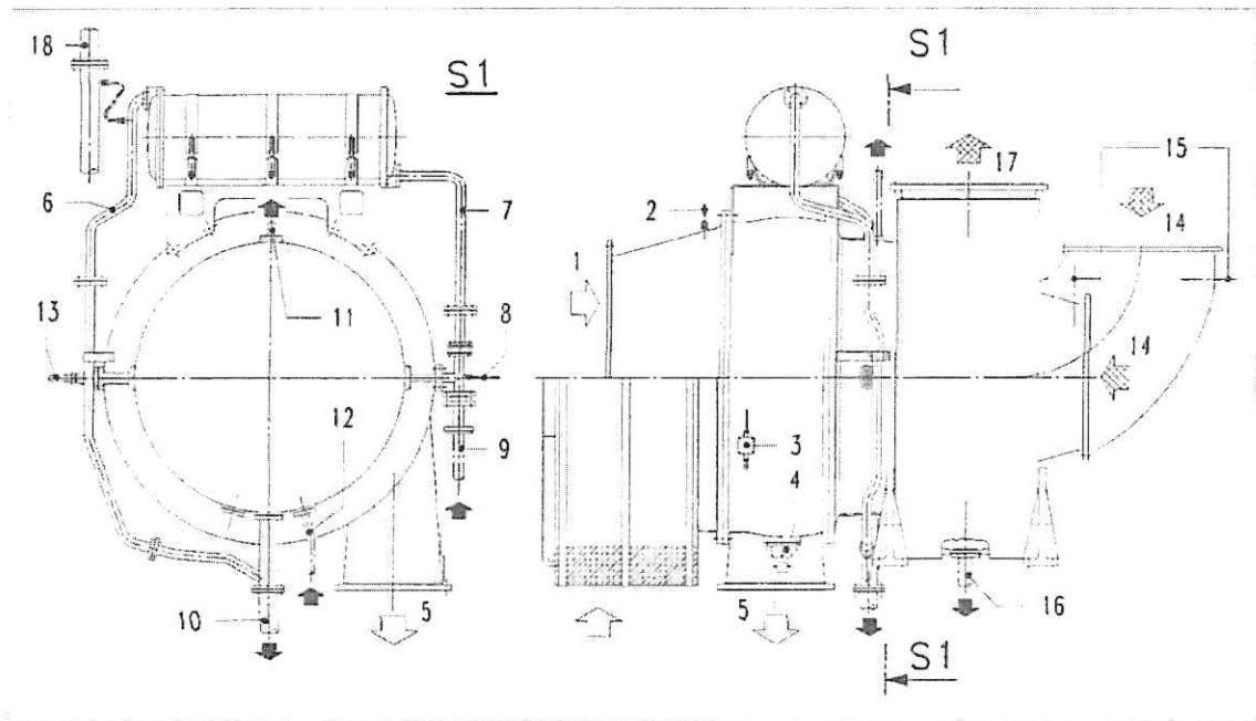
Figure 1: Connections on the turbocharger NA57/T9
