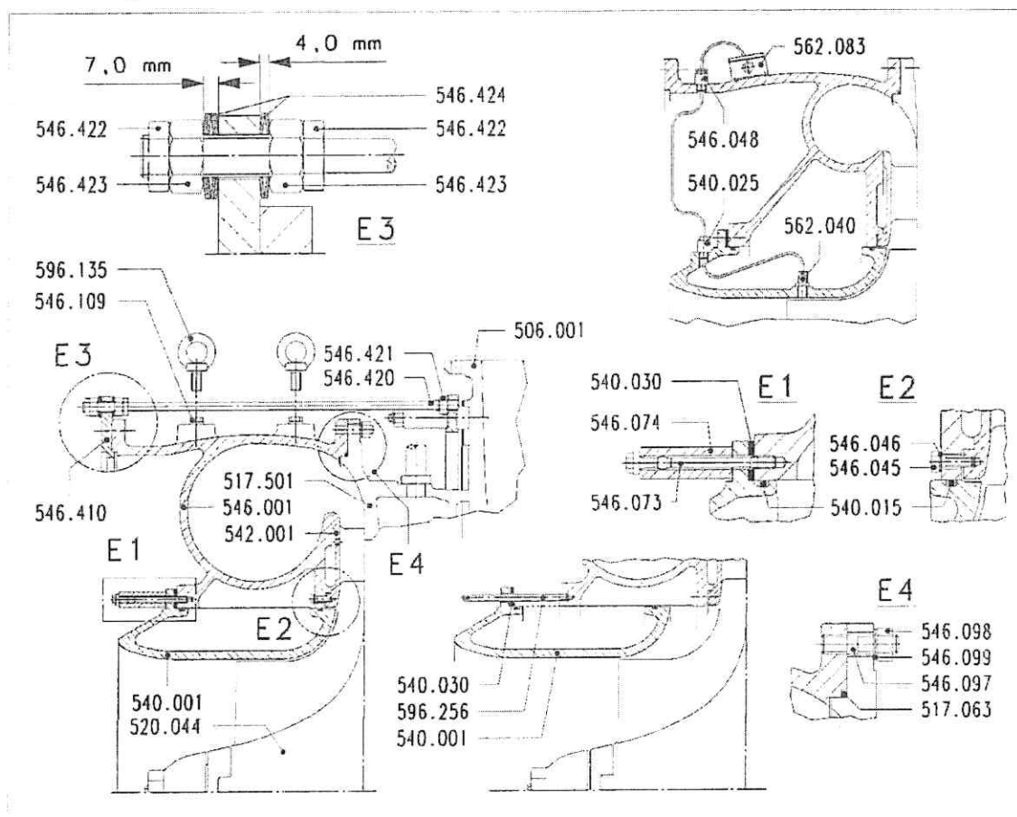
Figure 1: Removing and refitting the insert, speed transmitter, compressor casing, diffuser
