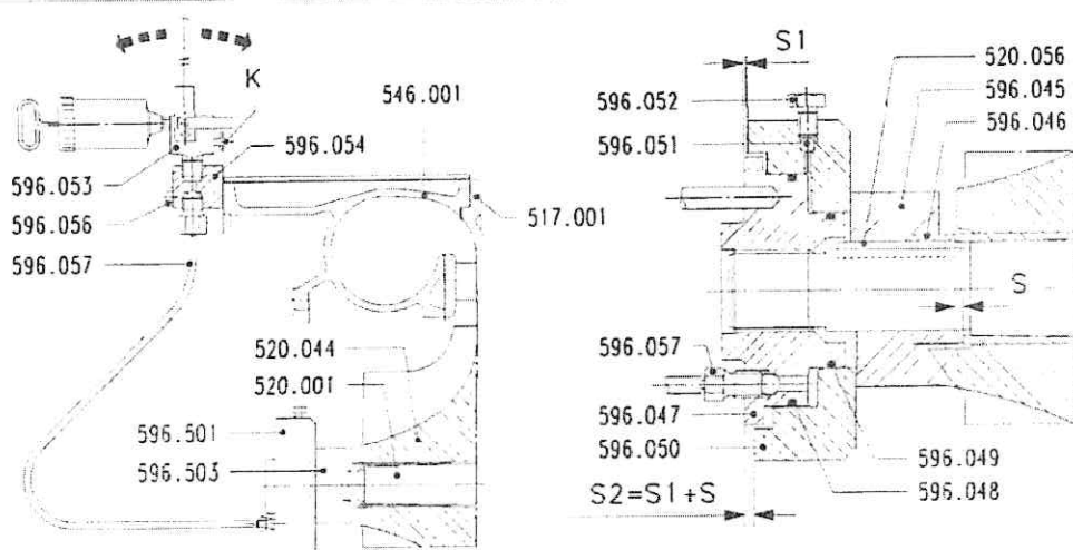
Figure 2: Refitting the compressor wheel
