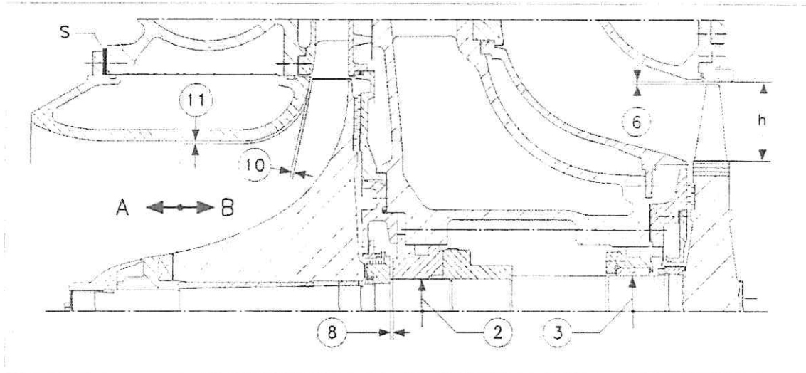
Figure 1: Gaps and clearances, measuring points
