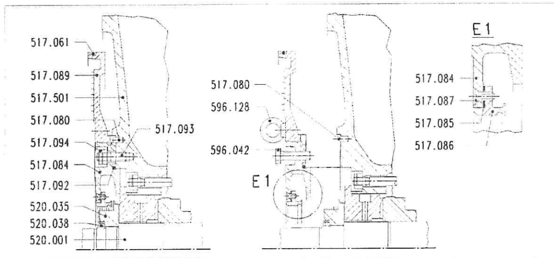
Figure 1: End cover and labyrinth disk, mounted on the bearing casing
