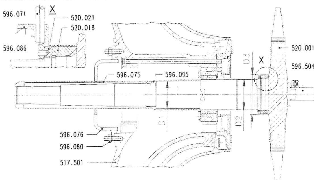
Figure 1: Removing, checking and refitting the turbine rotor
