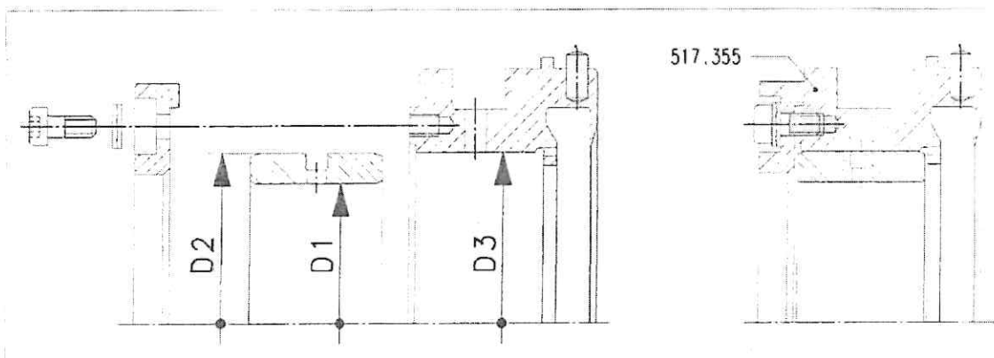
Figure 2: Checking the plain bearing (517.355)
