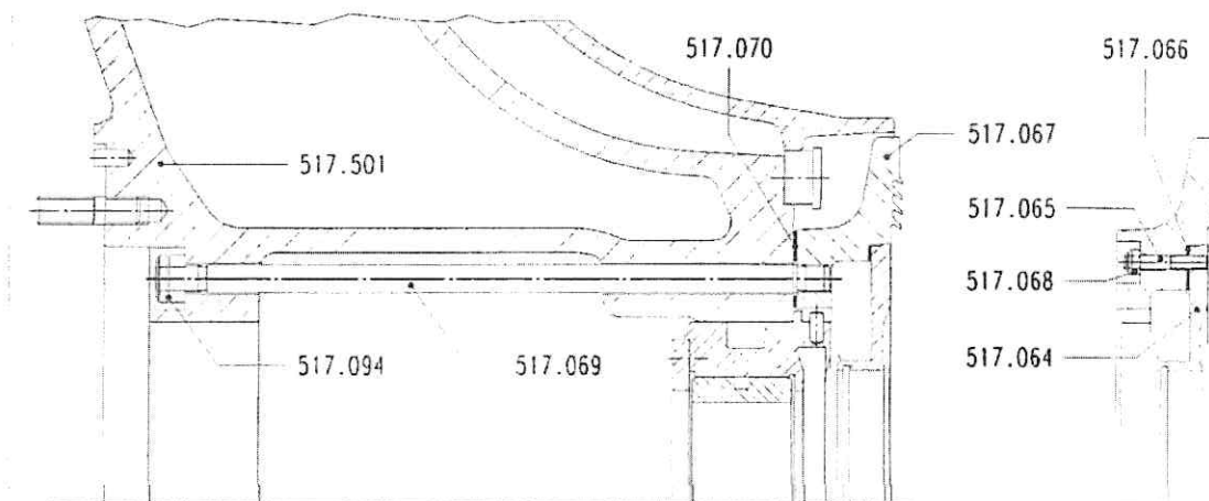
Figure 1: Removing and refitting the end cover and sealing cover
