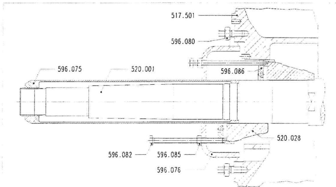
Figure 1: Removing and refitting the thrust ring
