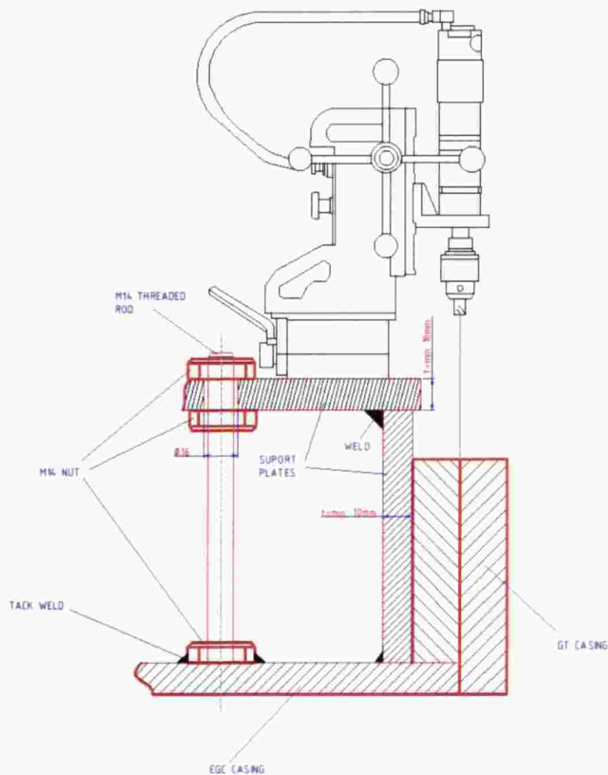
Figure 2. Sketch of hole drilling
