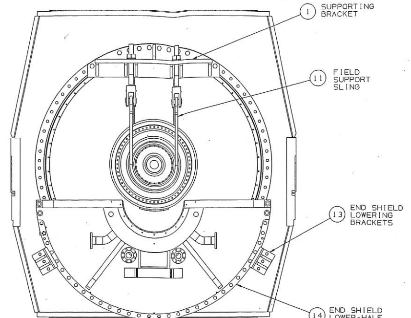
VIEW SHOWING FIELD SUPPORT AND SLING (COLLECTOR END)
