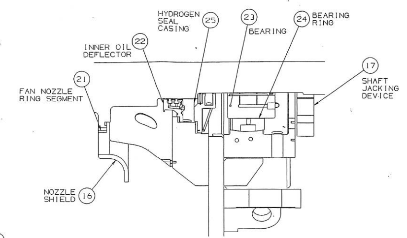
SECTION E-2 (F-7)
