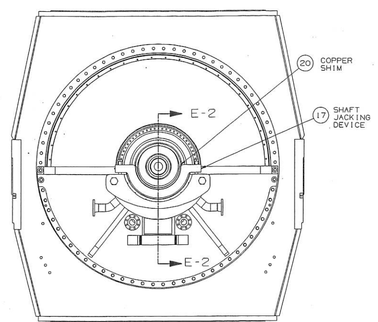
VIEW SHOWING SHAFT JACKING DEVICE (COLLECTOR AND TURBINE ENDS)
