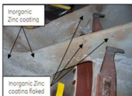
Figure 3: Inorganic zinc coating flaked from CDC strut
