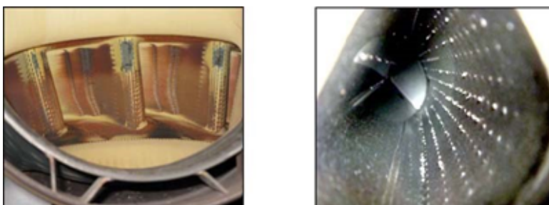
Figure 2: S1N distress at leading edge and clogged S1N cooling hole
