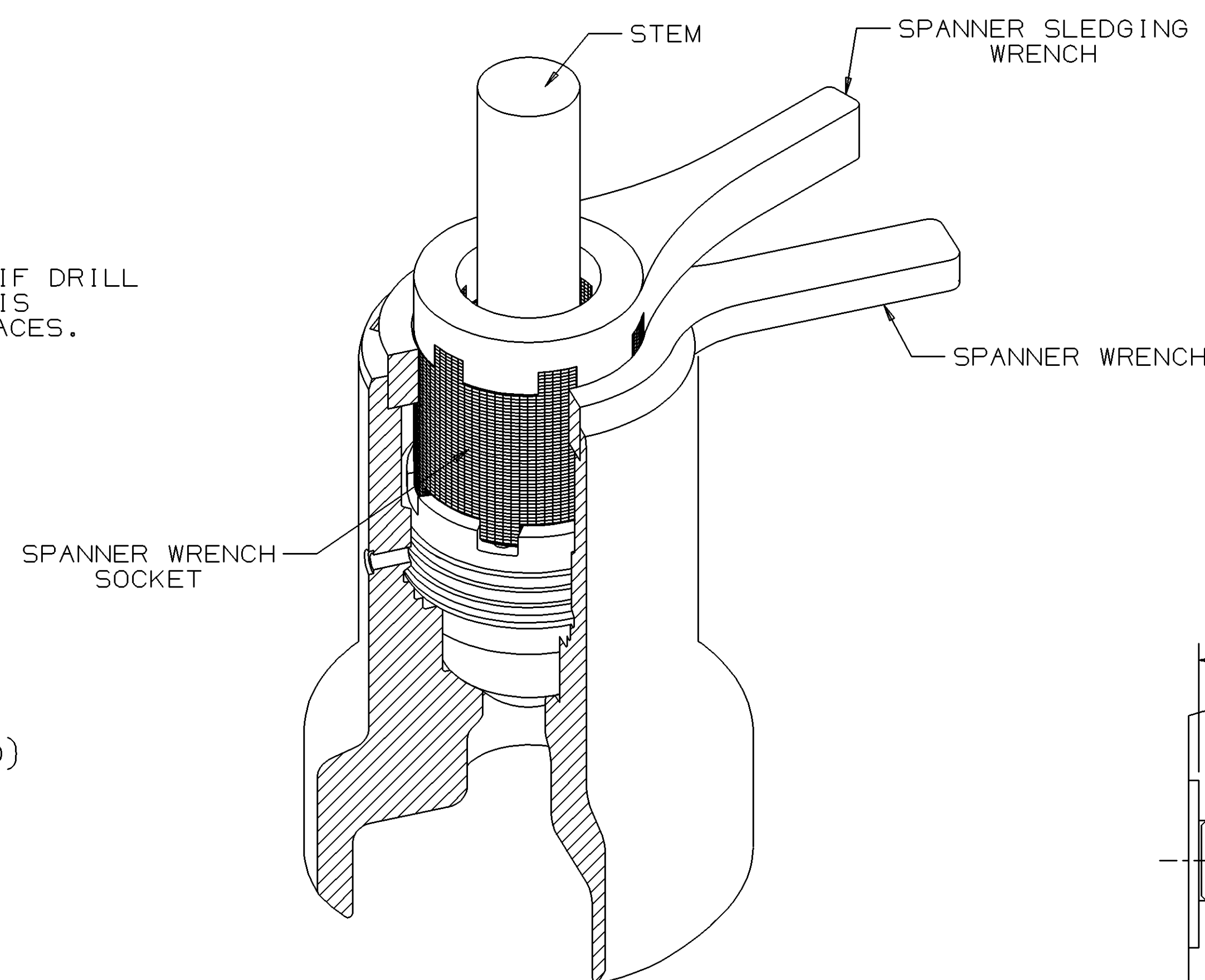
ISOMETRIC VIEW A-5
