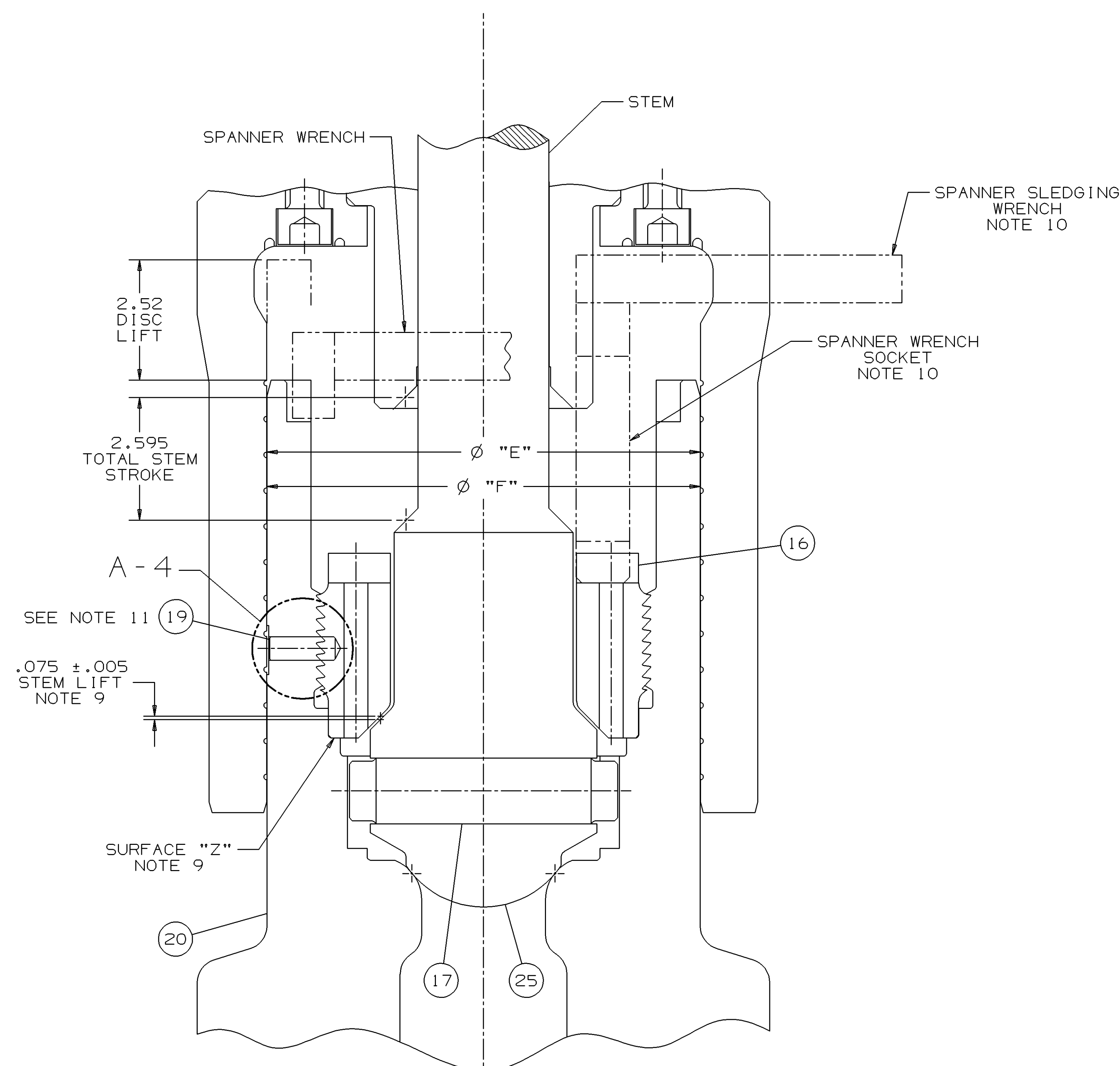
DETAIL B-3 (E-3 SHI)
