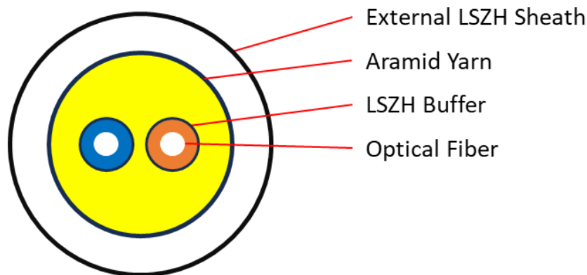
Figure 3 - Example of Indoor double-fiber cable structure
