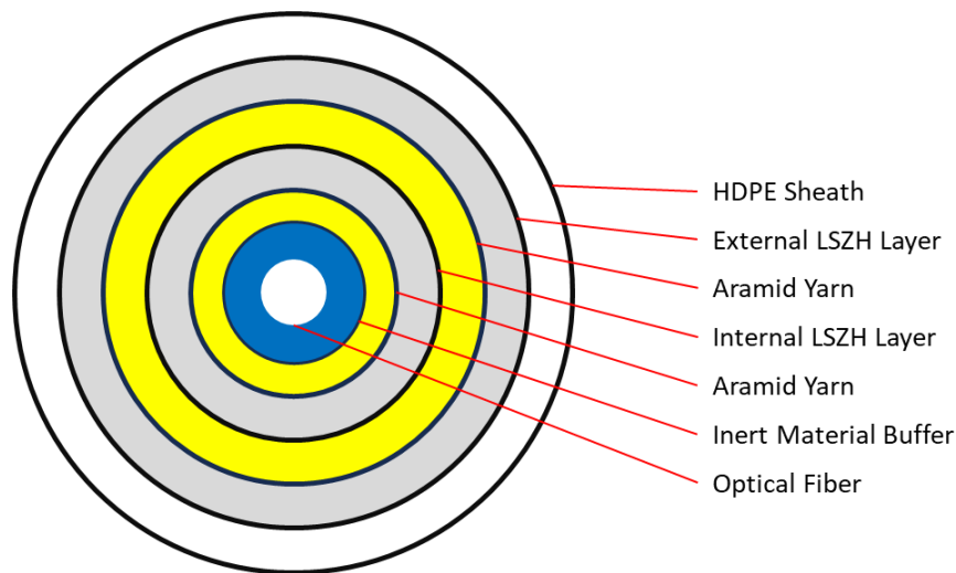
Figure 2 - Example of Outdoor single-fiber cable structure
