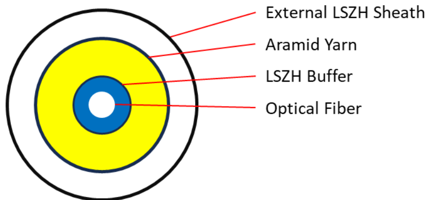
Figure 1 - Example of Indoor single-fiber cable structure
