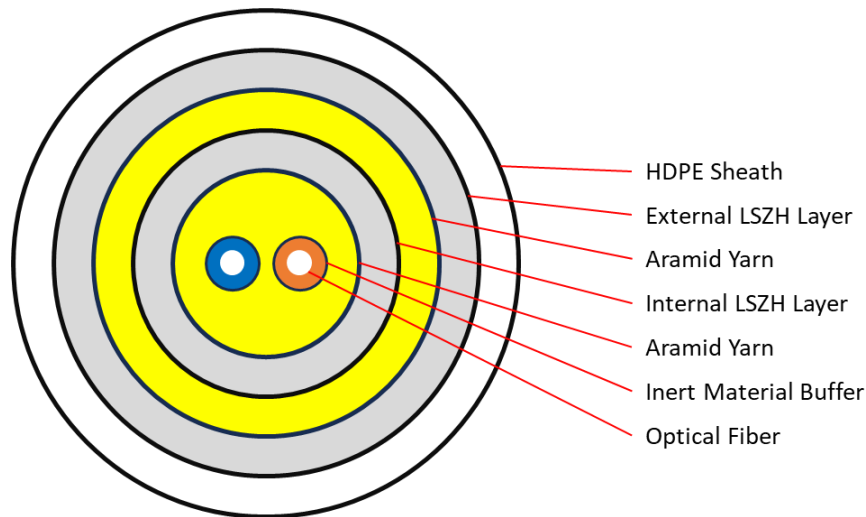
Figure 4 - Example of Outdoor double-fiber cable structure
