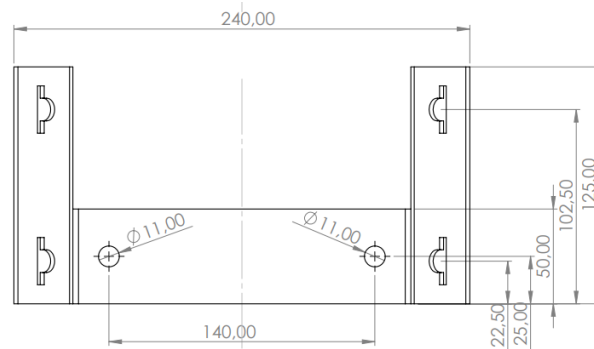
Figure 13 - Top view of U-shaped fiber slack storage pole distancer
