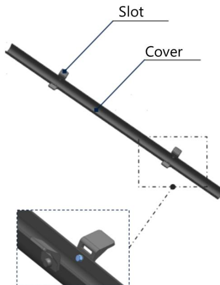
Figure 30 - Non Metallic Pole Cover
