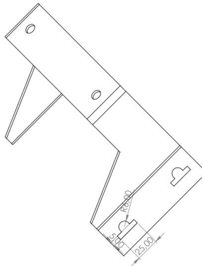
Figure 14 - Oblique view of U-shaped fiber slack storage pole distancer
