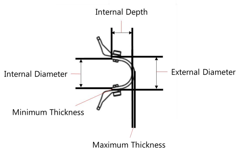
Figure 24 - Metal Pole Covers dimensions
