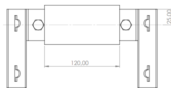
Figure 20 - Top view of Cable pole distancer
