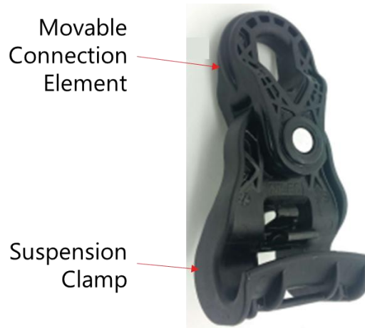
Figure 33 - Suspension Clamps for ABC and ADSS cables
