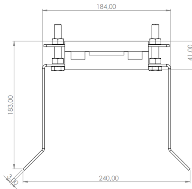
Figure 19 - Front view of Cable pole distancer
