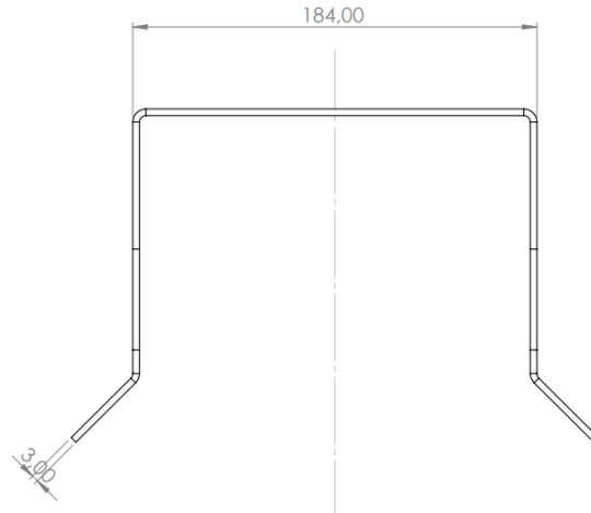
Figure 12 - Front view of U-shaped fiber slack storage pole distancer
