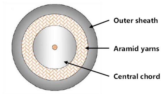
Figure 35 - Dielectric rope
