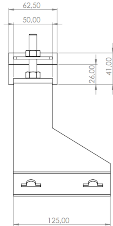
Figure 18 - Side view of Cable pole distancer
