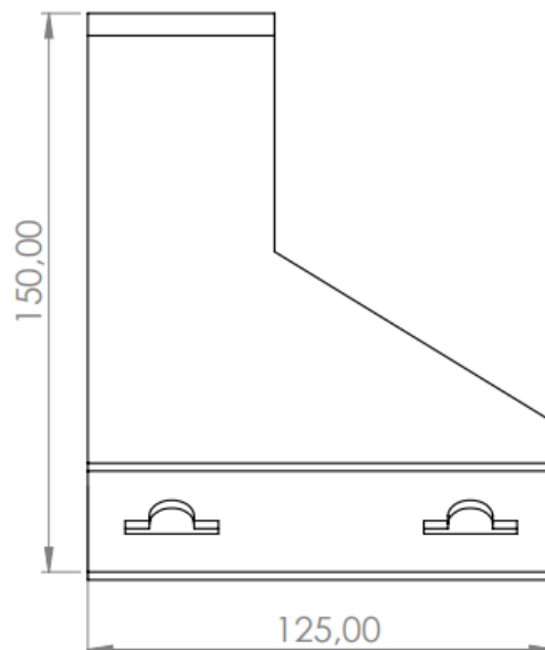
Figure 11 - Side view of U-shaped fiber slack storage pole distancer
