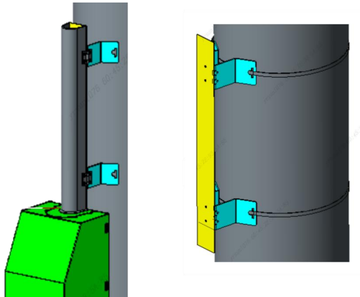
Figure 31 - Example of Non Metallic Pole Covers with Back Protection installed on pole
