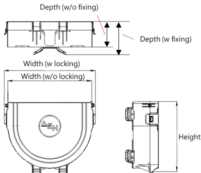
Figure 6 - Dimensions of U-shaped fiber slack storage device
