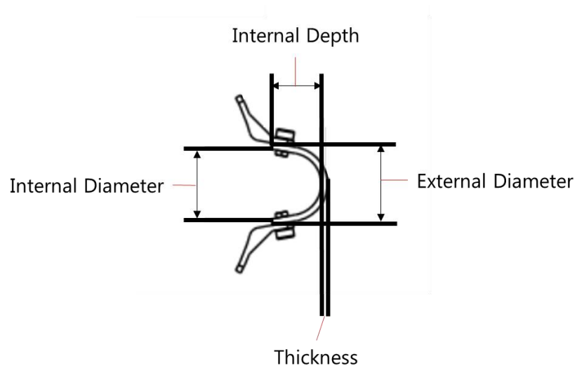
Figure 27 - MV Cover Protectors dimensions
