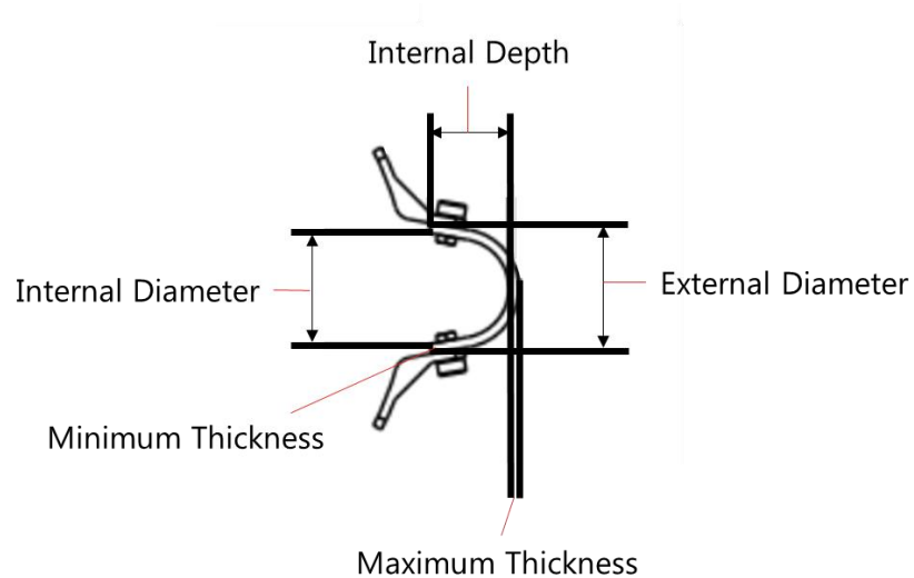
Figure 29 - Non Metallic Pole Covers dimensions
