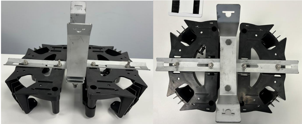
Figure 2 - Example of Fiber slack storage pole distancer
