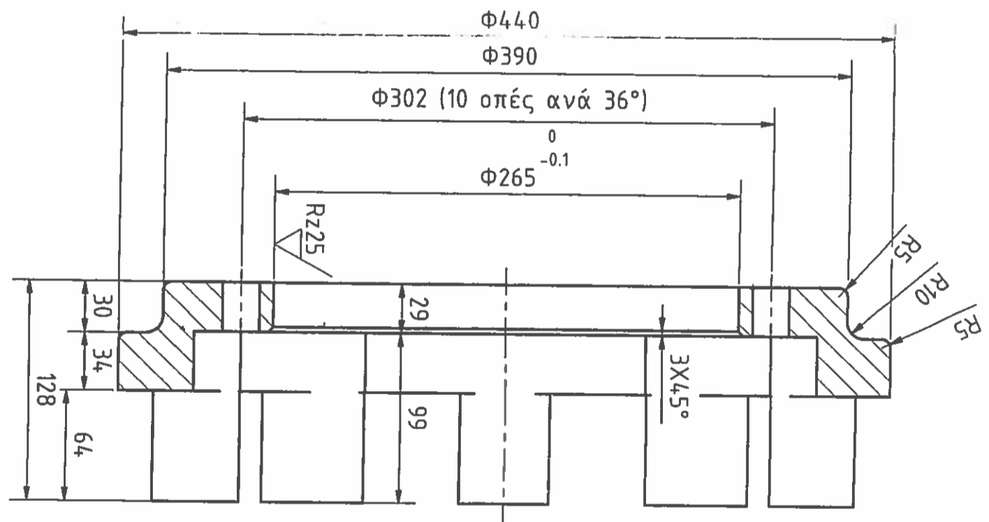
F-F (1:3)
