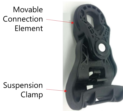
Figure 19 - Suspension Clamps for ABC and ADSS cables
