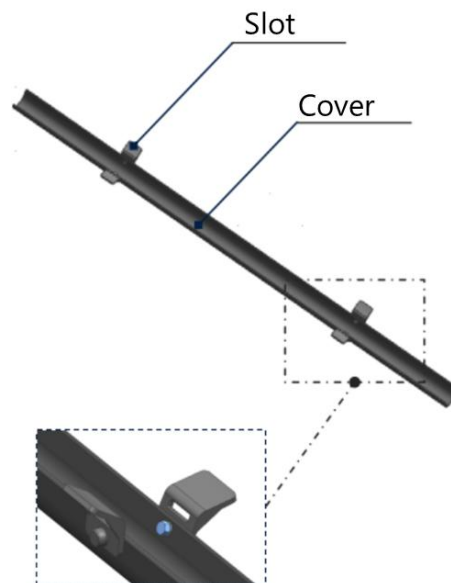
Figure 16 - Non Metallic Pole Cover
