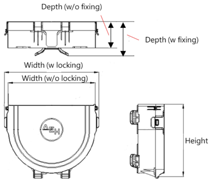
Figure 5 - Dimensions of U-shaped fiber slack storage device
