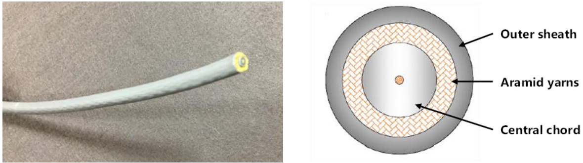
Figure 21 - Dielectric rope
