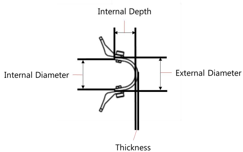
Figure 13 - MV Cover Protectors dimensions
