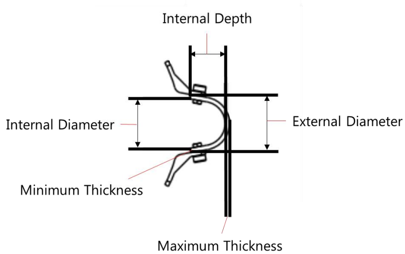
Figure 15 - Non Metallic Pole Covers dimensions
