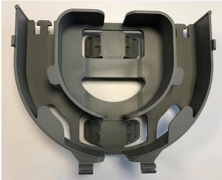
Figure 6 - Example of PP+GF U-shaped slack storage internal configuration
