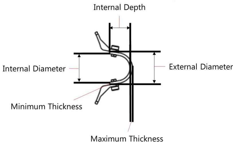
Figure 10 - Metal Pole Covers dimensions
