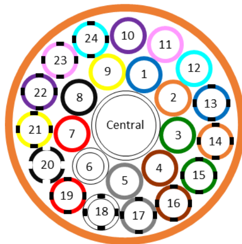
Figure 11 - Example of 24x4/7+1x10/14 DB Microducts Bundle
