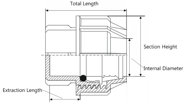
Figure 13 - End Cap for HDPE Ducts dimensions
