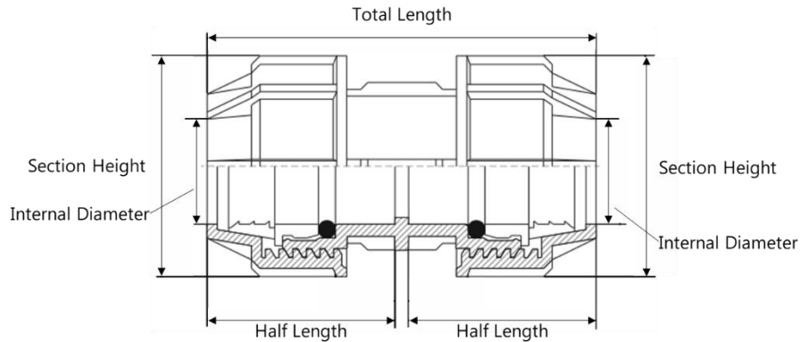
Figure 16 - Connector for HDPE Ducts dimensions
