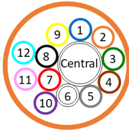
Figure 9 - Example of 12x4/7+1x10/14 DB Microducts Bundle
