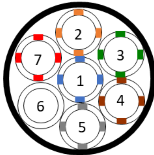
Figure 8 - Example of 7x8/10 DI Microducts Bundle
