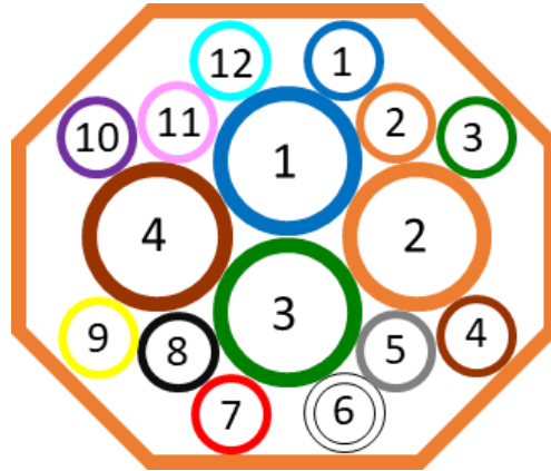
Figure 10 - Example of 12x4/7+4x10/14 DB Microducts Bundle
