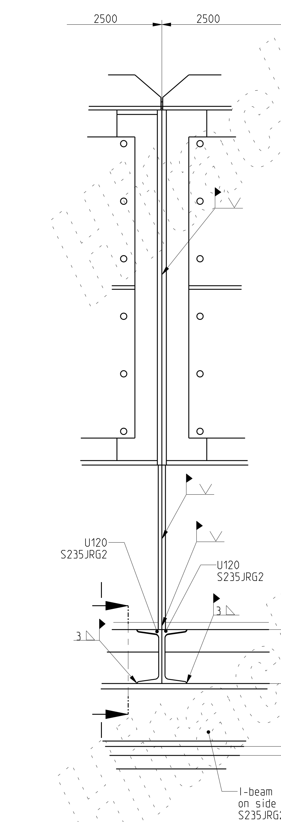
Mounting on platform/ Connection between trough
