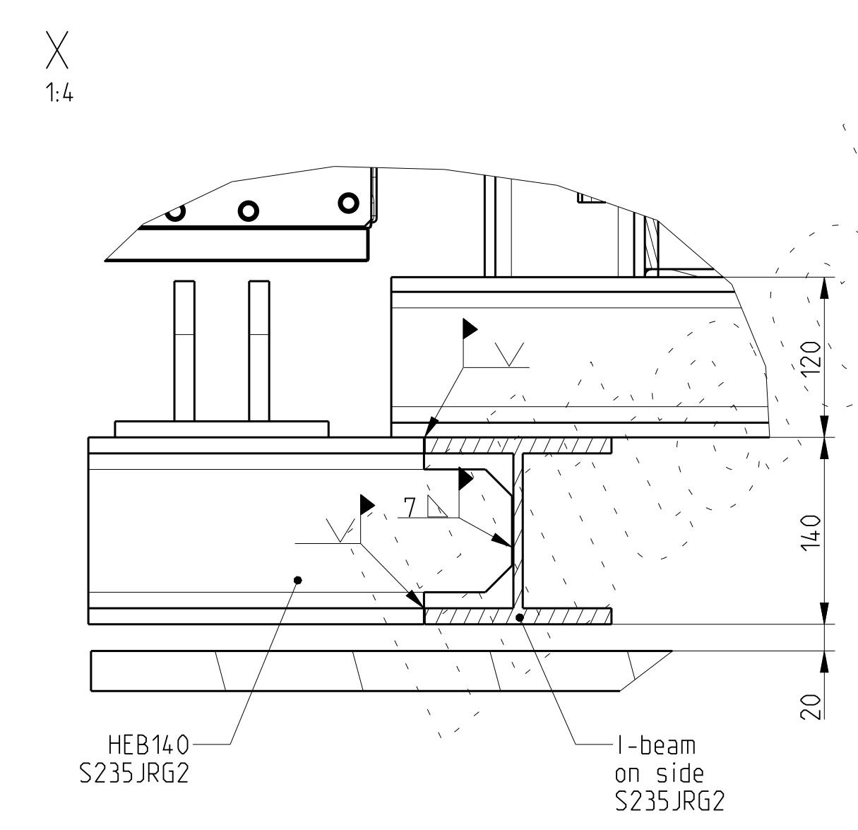
Torque Arm
