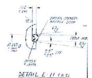
DETAIL E-11 (B-7)
