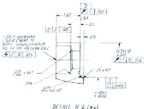
DETAIL H-6 (B-6)
