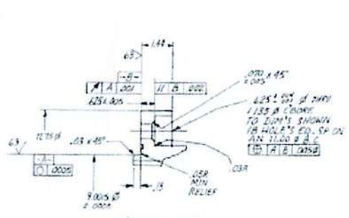
DETAIL H-2 (B-2)
