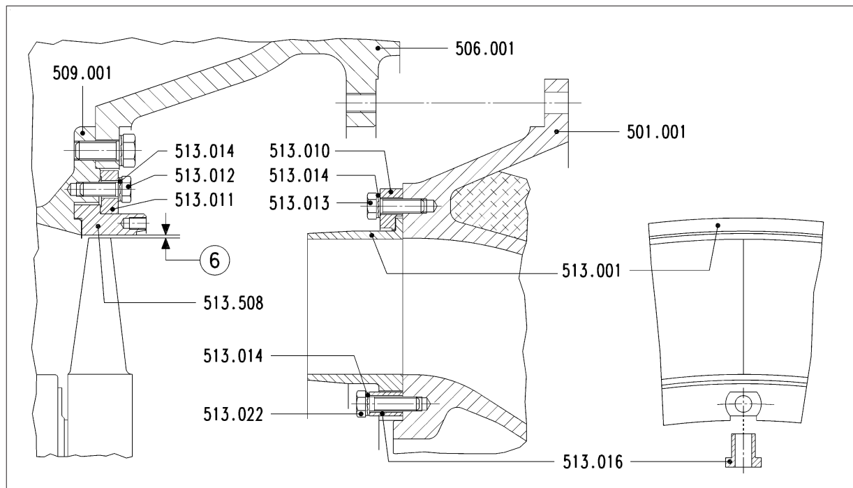
Figure 1: Removing and refitting the nozzle ring and shroud ring
