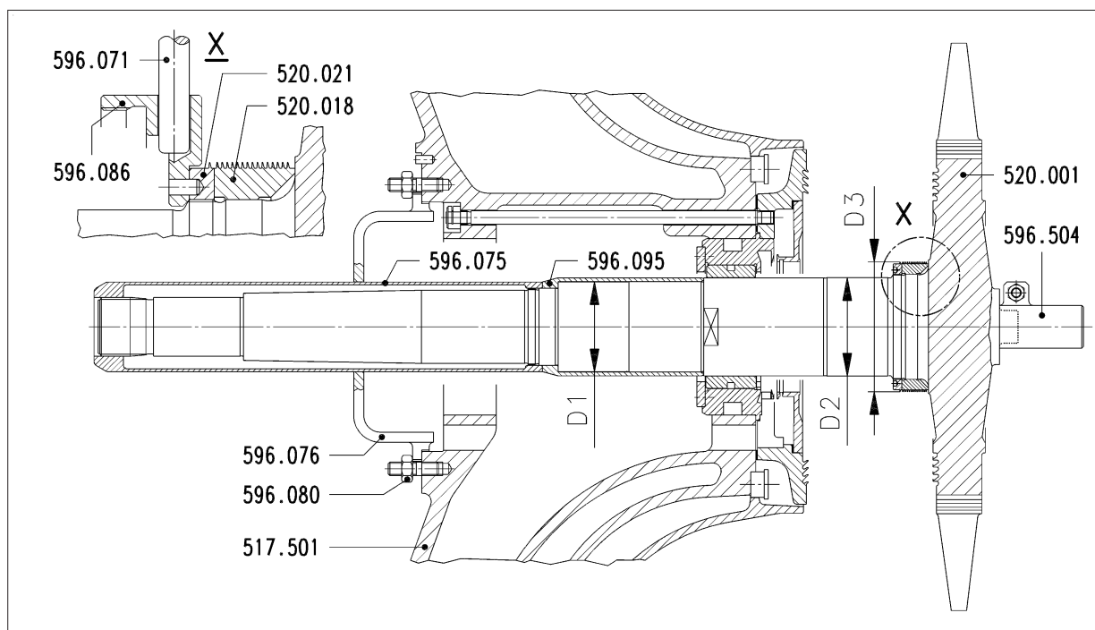
Figure 1: Removing, checking and refitting the turbine rotor
