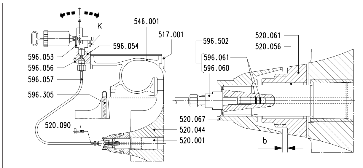
Figure 1: Removing the compressor wheel
