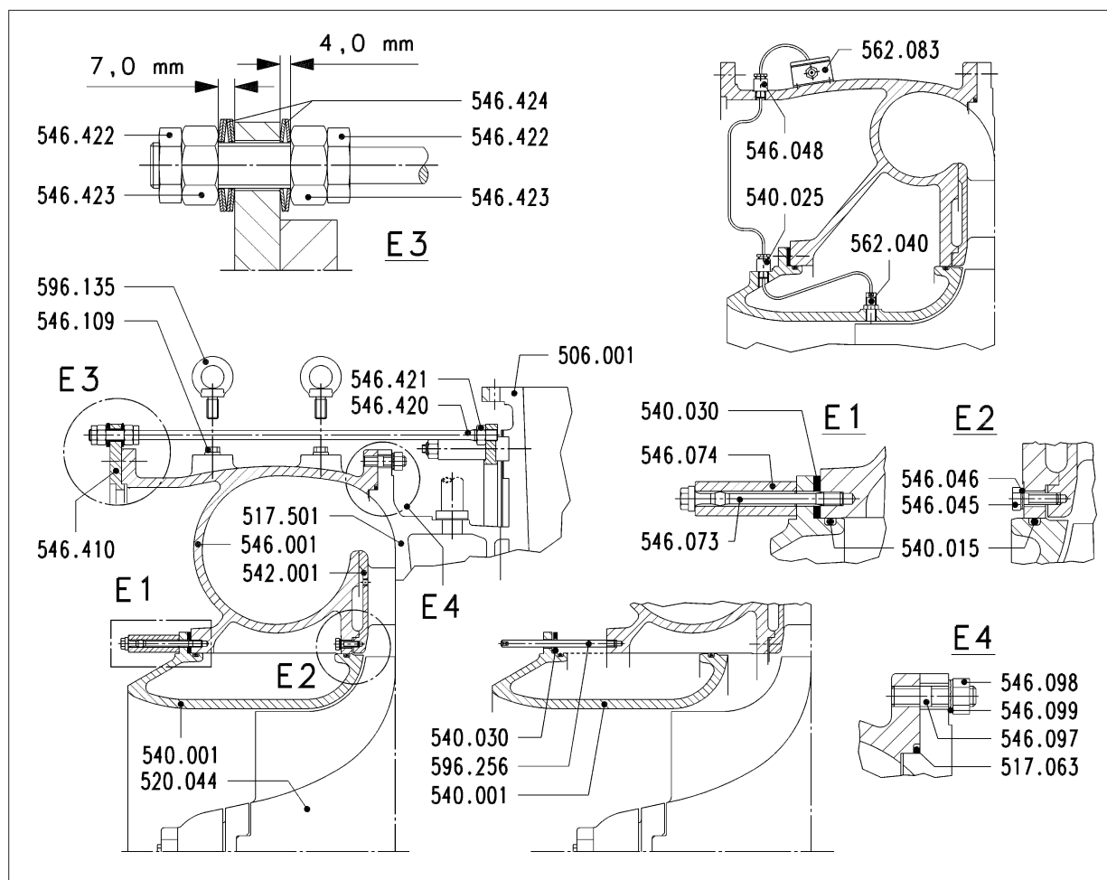
Figure 1: Removing and refitting the insert, speed transmitter, compressor casing, diffuser
