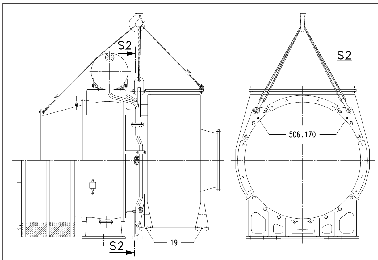
Figure 2: Removing and refitting the complete turbocharger NA57/T9
