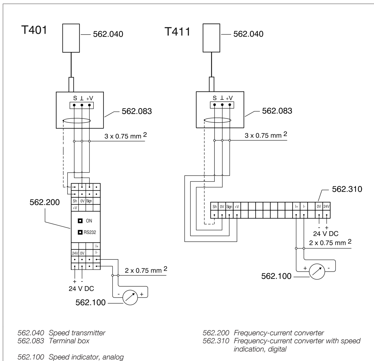
Figure 3: Cable connection of the speed measuring device
