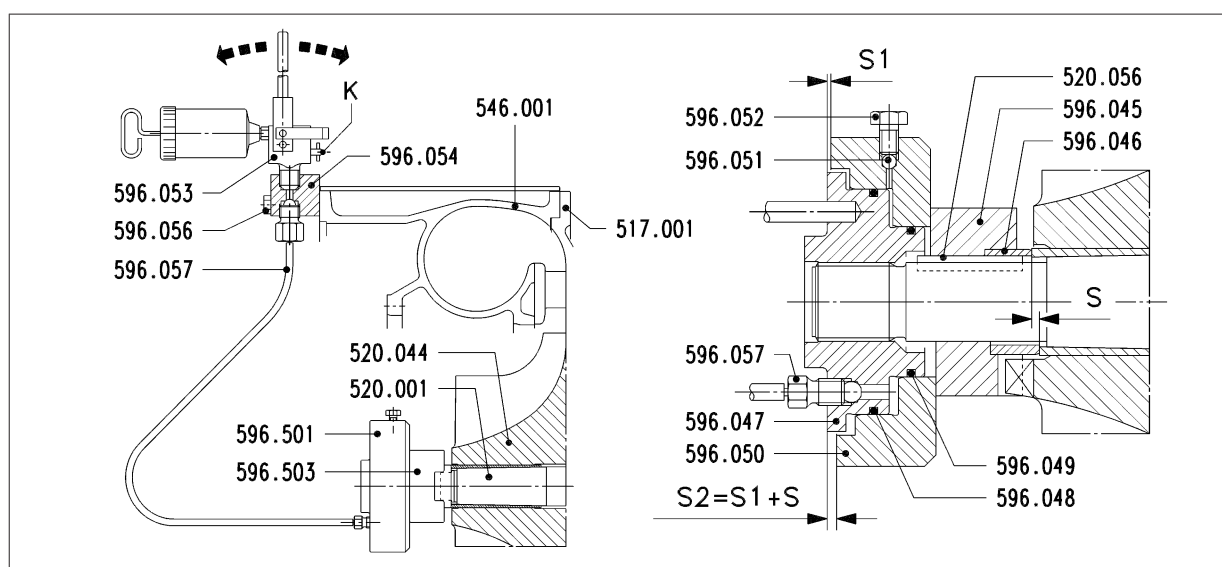
Figure 2: Refitting the compressor wheel
