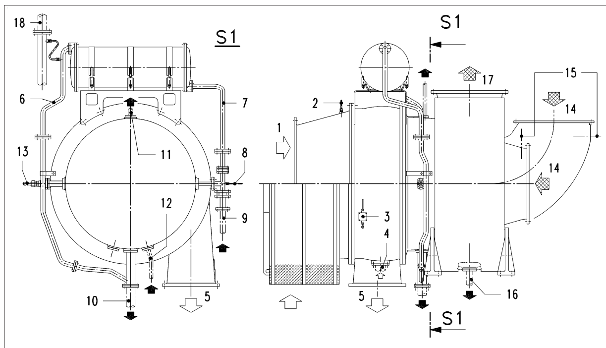
Figure 1: Connections on the turbocharger NA57/T9
