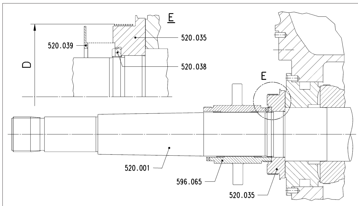
Figure 1: Removing, checking and refitting the locating ring
