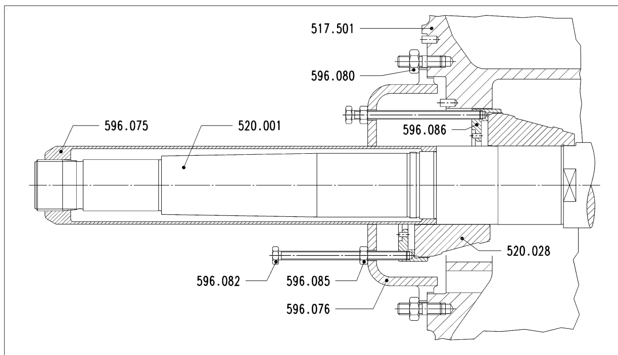
Figure 1: Removing and refitting the thrust ring
