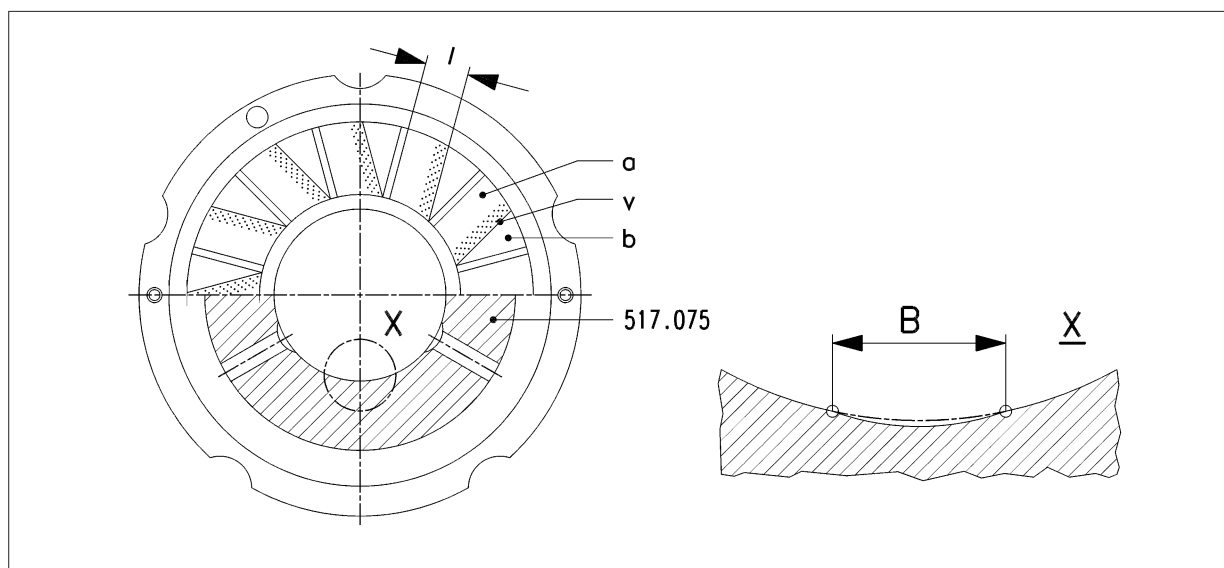
Figure 1: Checking the locating bearing (517.075)
