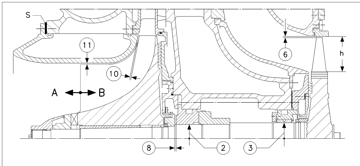
Figure 1: Gaps and clearances, measuring points
