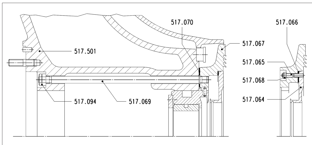
Figure 1: Removing and refitting the end cover and sealing cover
