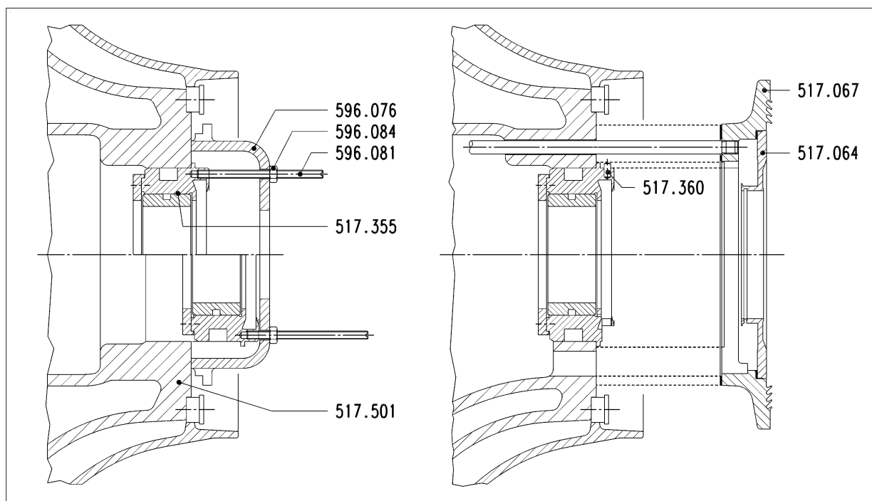
Figure 1: Removing and refitting the plain bearing
