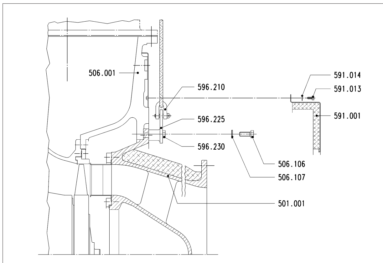
Figure 1: Removing and refitting the gas admission casing
