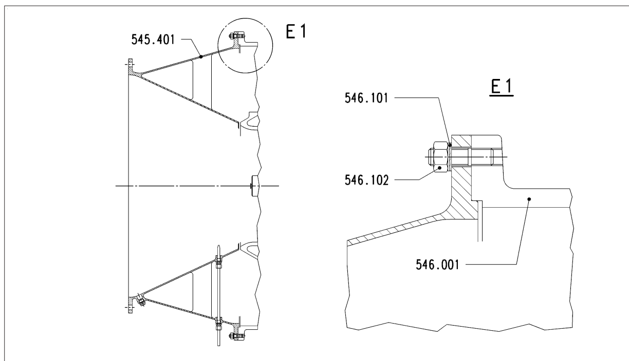
Figure 1: Removing and refitting the air intake casing
