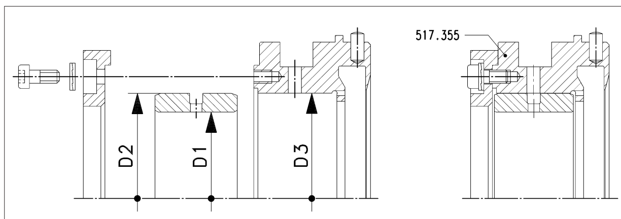
Figure 2: Checking the plain bearing (517.355)
