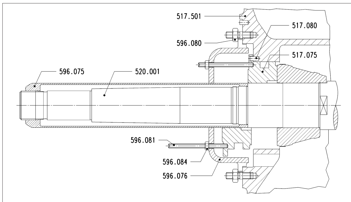
Figure 1: Removing and refitting the locating bearing
