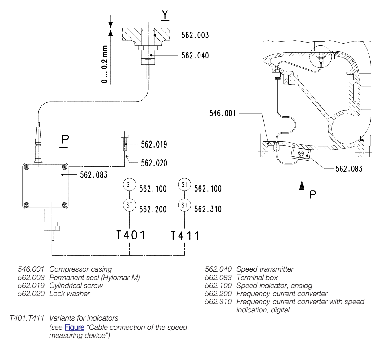
Figure 2: Speed measuring device
