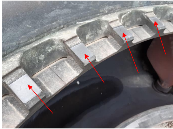
Turbine Suspension Ring – fretting contact surface (2-3mm)
