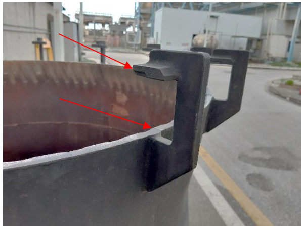
Typical Fretting Belt Seals Hooks and top contact surface
