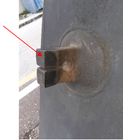
Side Guiding Keys – Hard Face Coating
