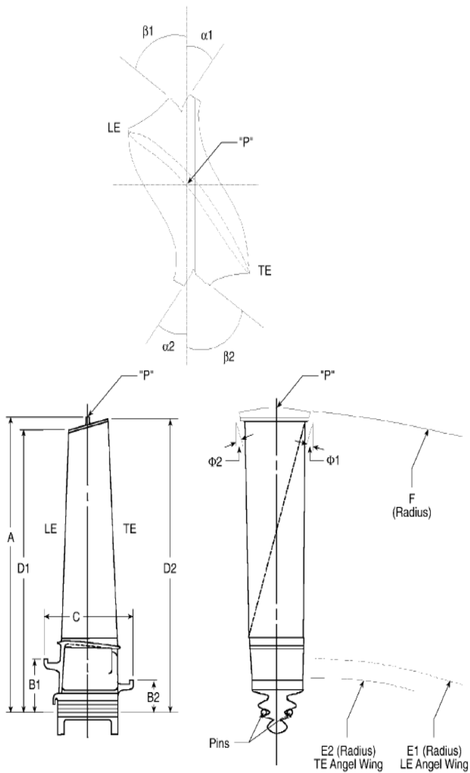
Form I-A GE MS7001 Model F/FA Third Stage Bucket Dimensional Inspection Form
