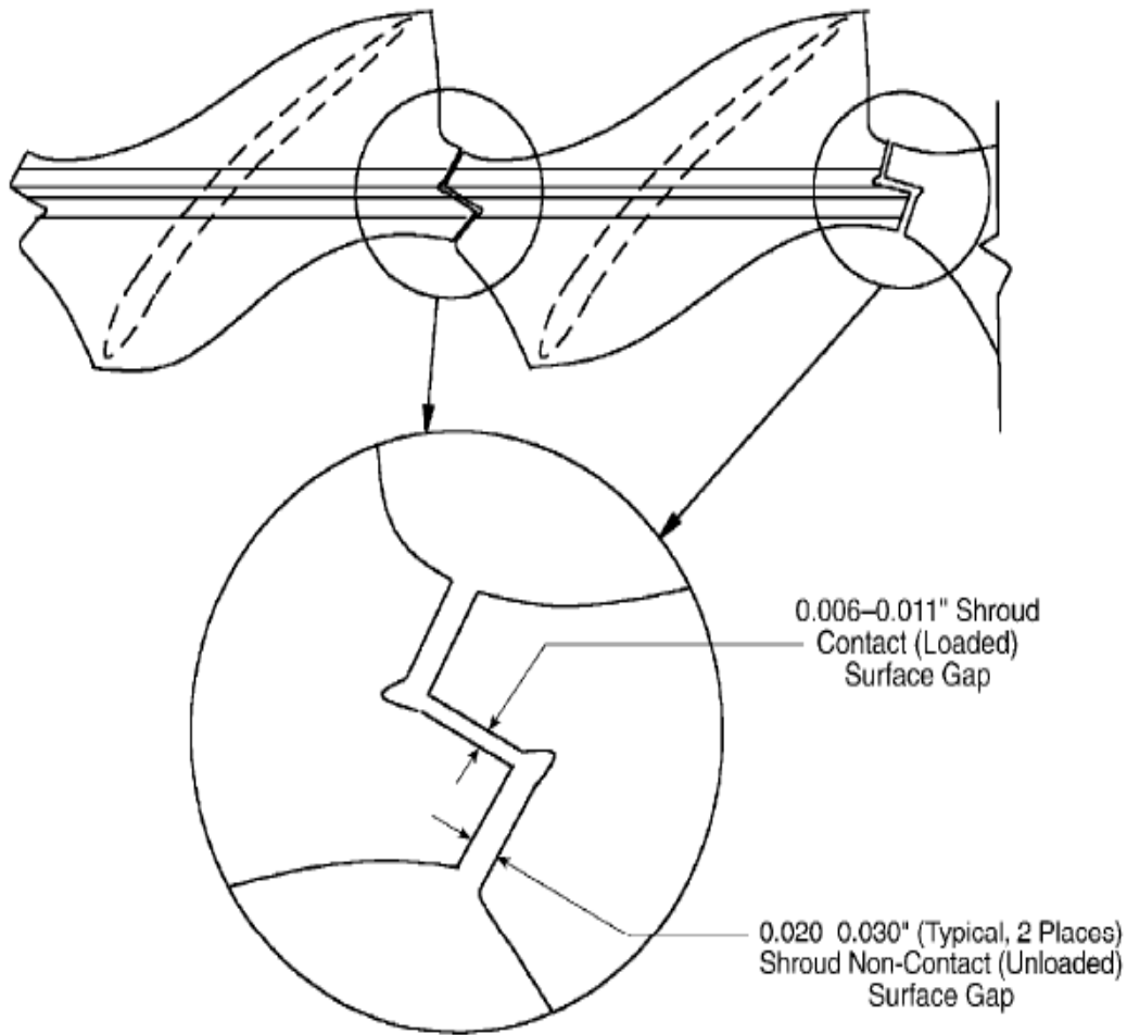
Shroud Z-Notch Gap Check
