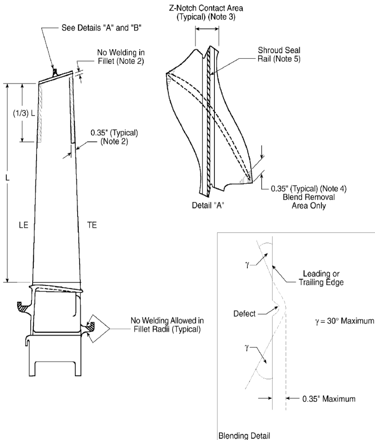
Figure 7-1 GE MS7001 Model F/FA Third Stage Bucket Weld and Blend Repairs (Welding/Blending Allowed in Shaded Regions Only)
