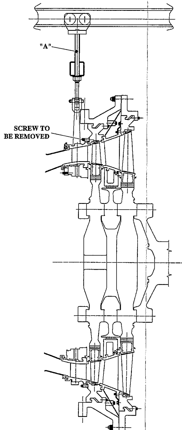
FIG. 5.21 - DISASSEMBLY OF 1ST STAGE NOZZLES ASSEMBLY
