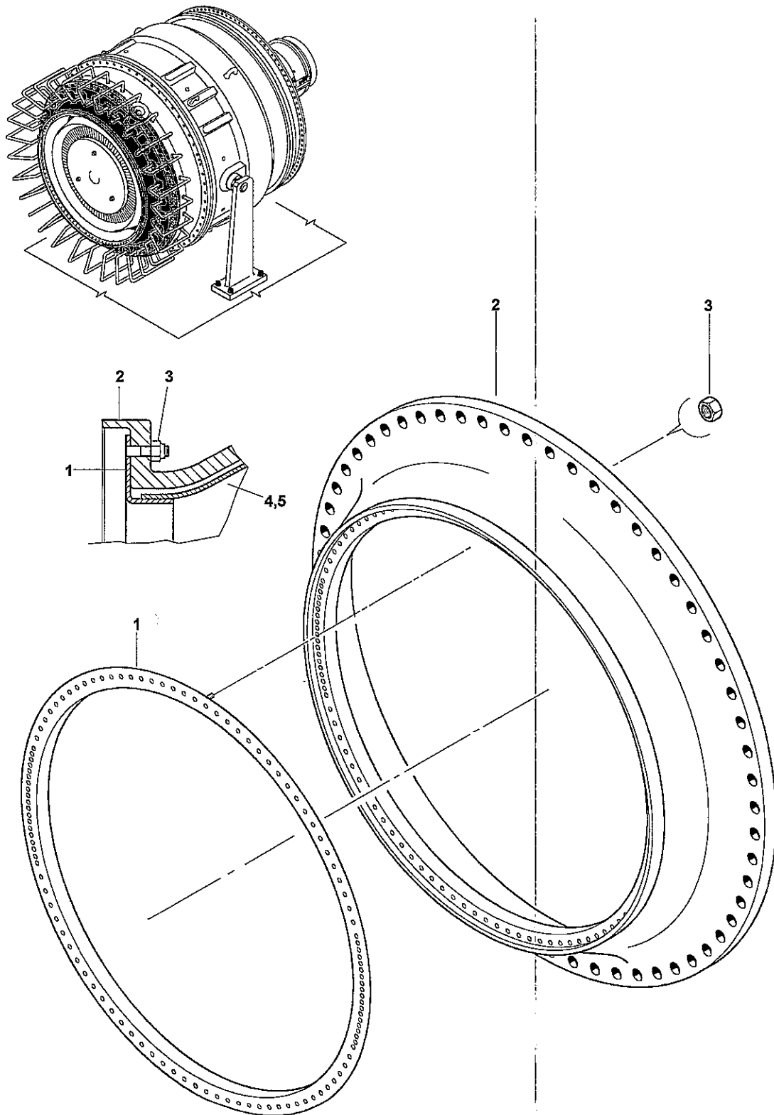
Figure 4 - Transition Case
