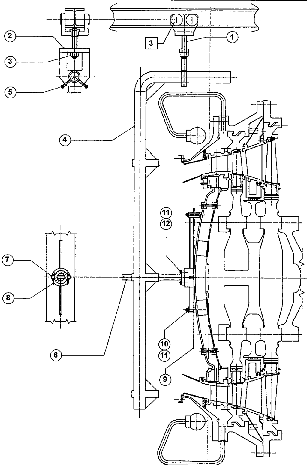
FIG. 5.13 - DISASSEMBLY OF BONDING BAFFLE
