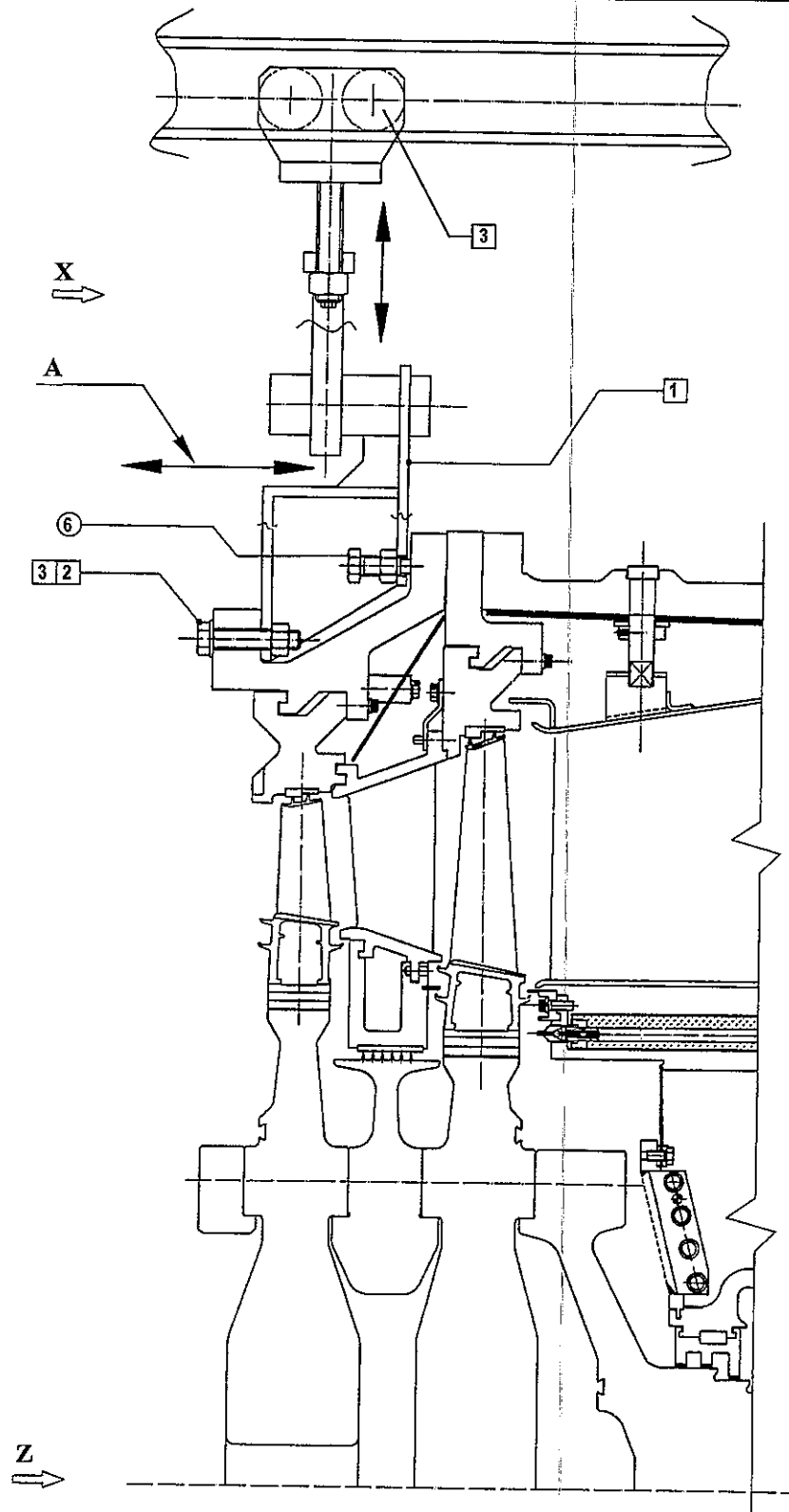
FIG. 5.23 - DISASSEMBLY OF 1ST STAGE TURBINE CASING
