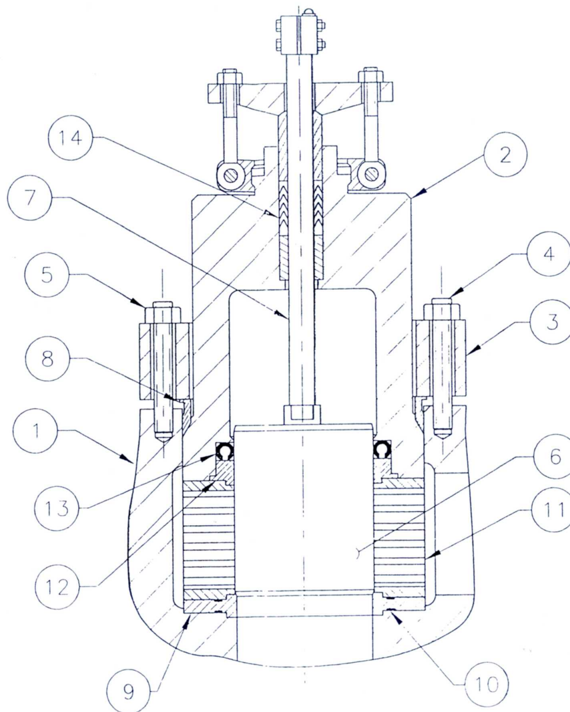
BODY - SECTIONAL VIEW
