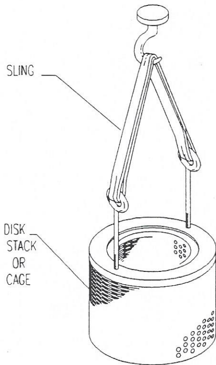
DISK STACK LIFTING ARRANGEMENT
