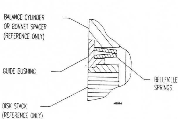
BELLEVILLE SPRING CONFIGURATION
