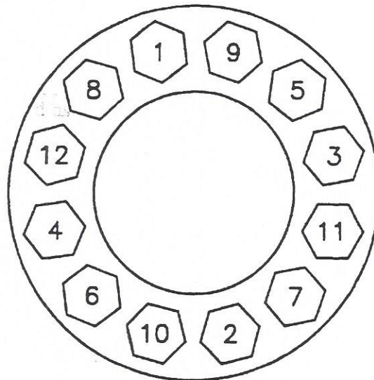
TORQUE PATTERN
