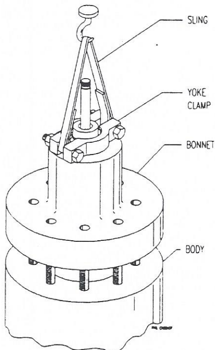
BONNET LIFTING ARRANGEMENT
