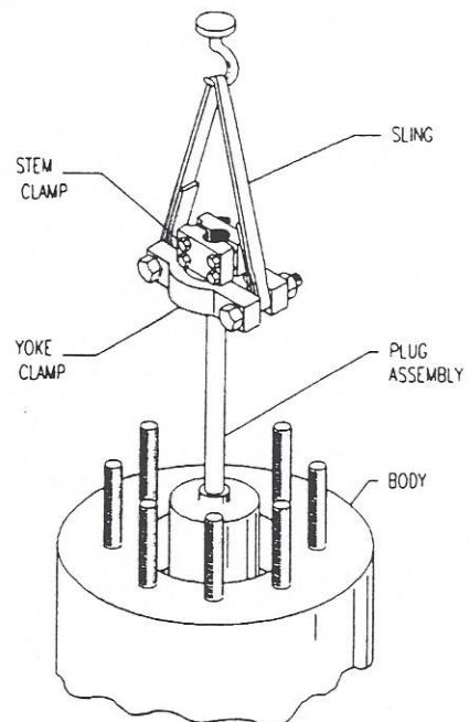
PLUG ASSEMBLY LIFTING ARRANGEMENT
