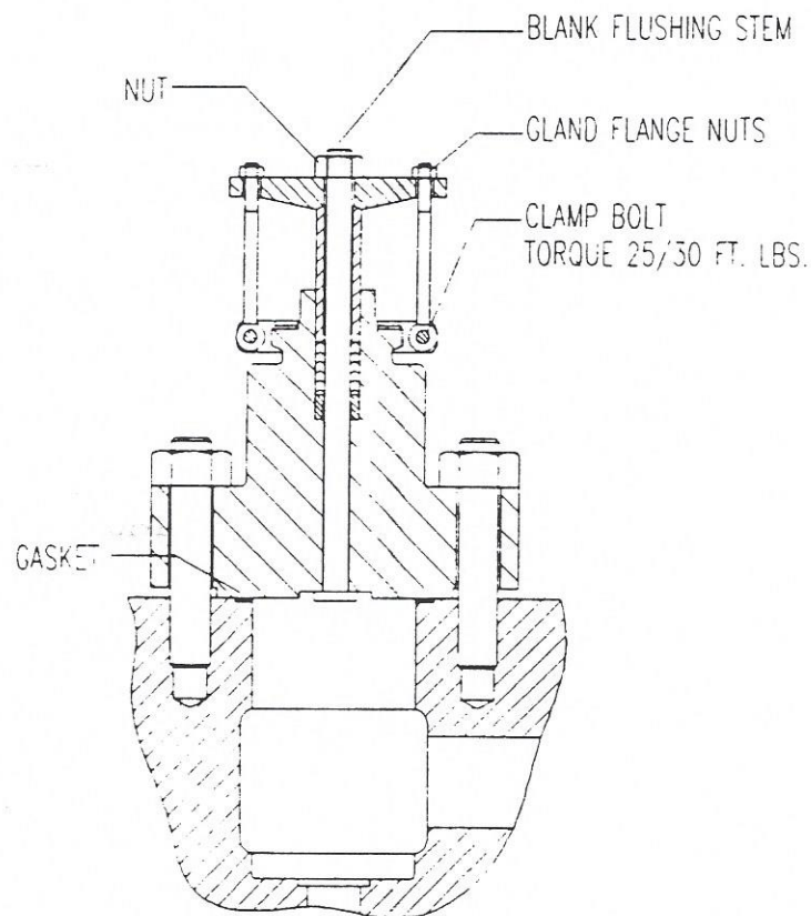
FLUSHING TRIM
