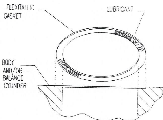
UPPER GASKET INSTALLATION
