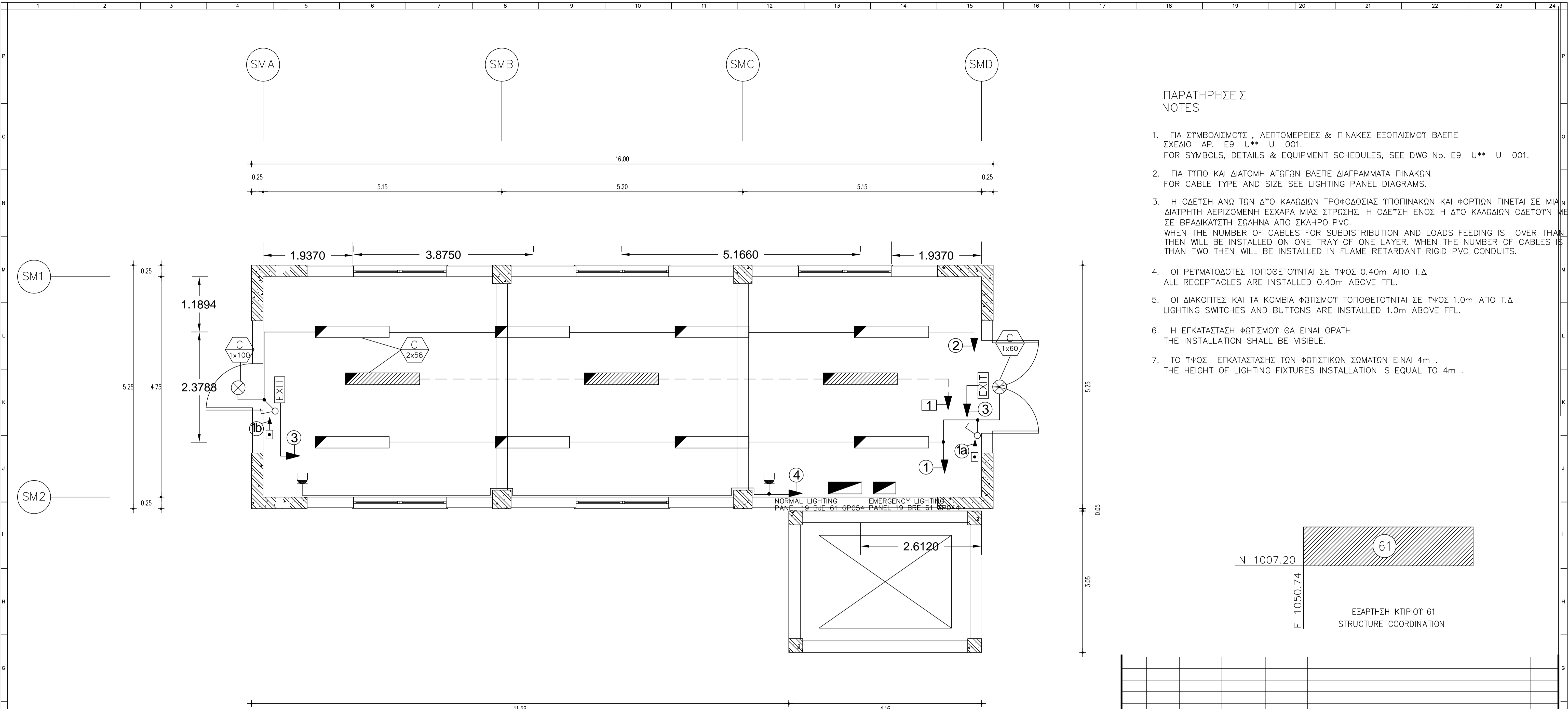
ΚΑΤΟΨΗ ΙΣΟΓΕΙΟΥ GROUND FLOOR PLAN KL 1:50 SC.
