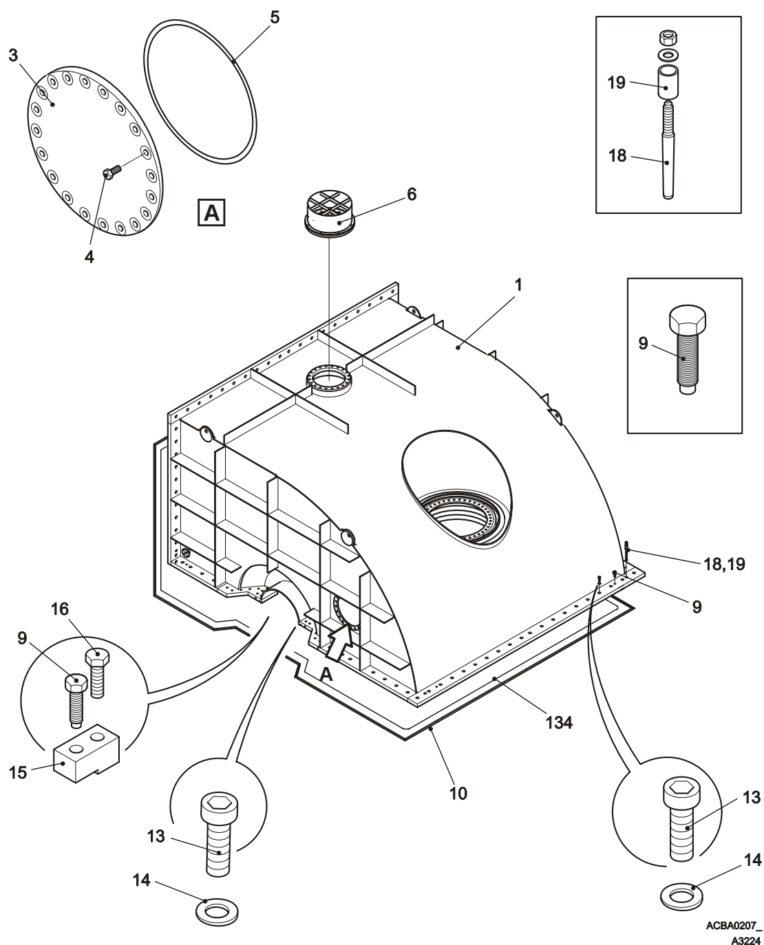
Fig.1 Outer casing, upper half
