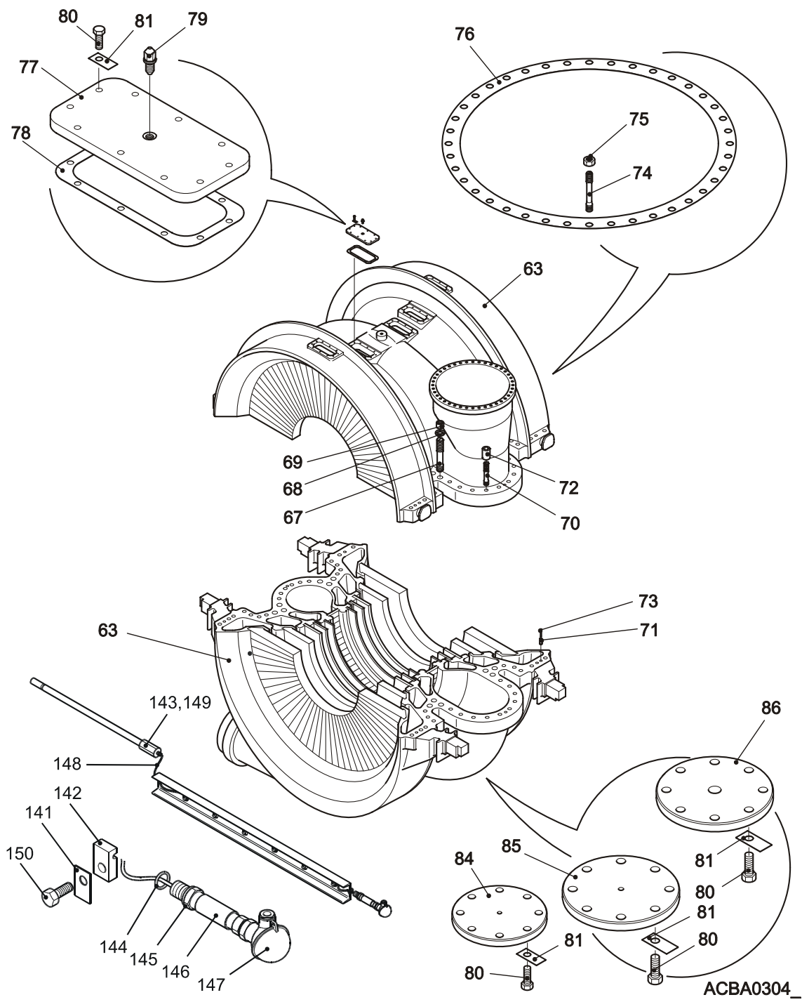
Fig.3 Inner casing
