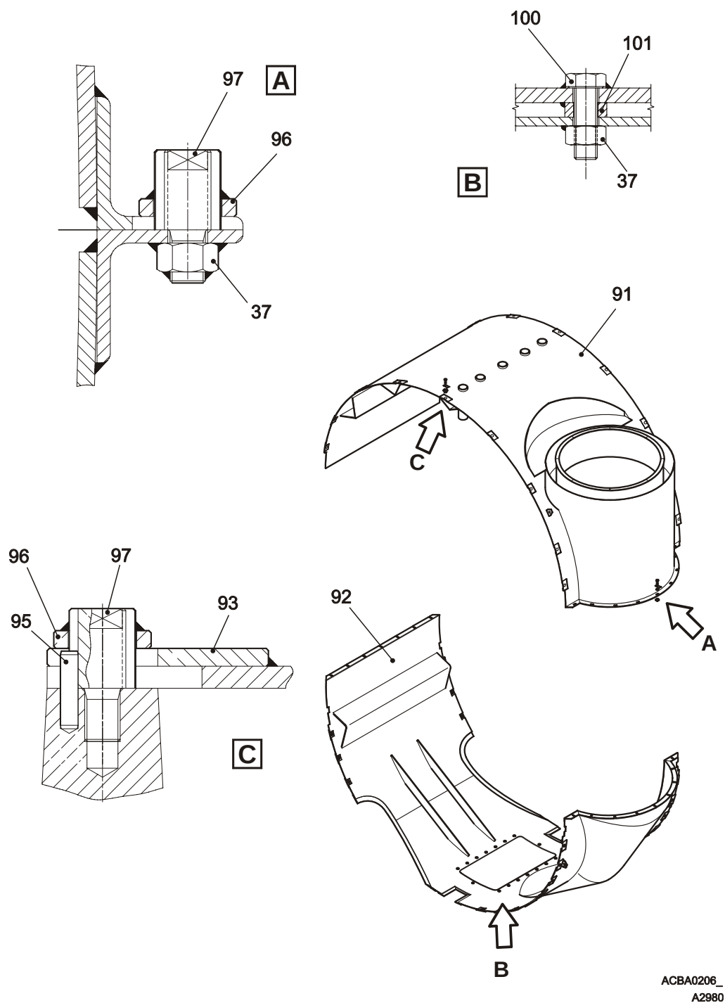
Fig.4 Inner casing, shielding
