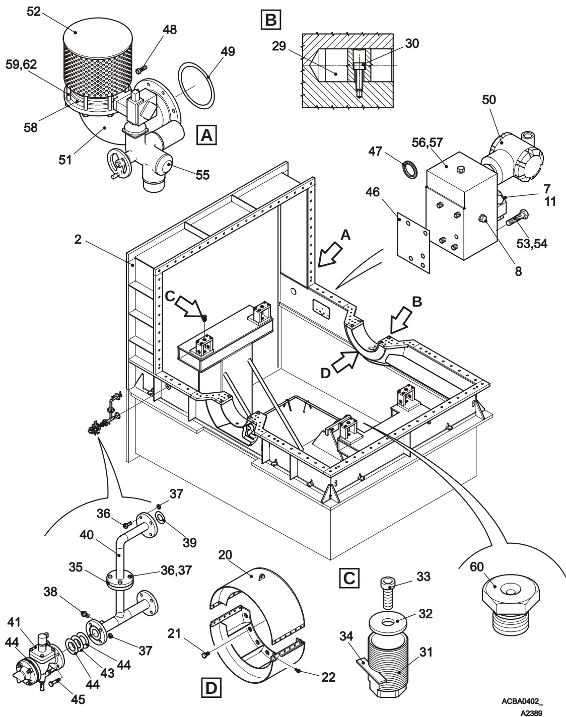
Fig. 2 Outer casing, lower half
