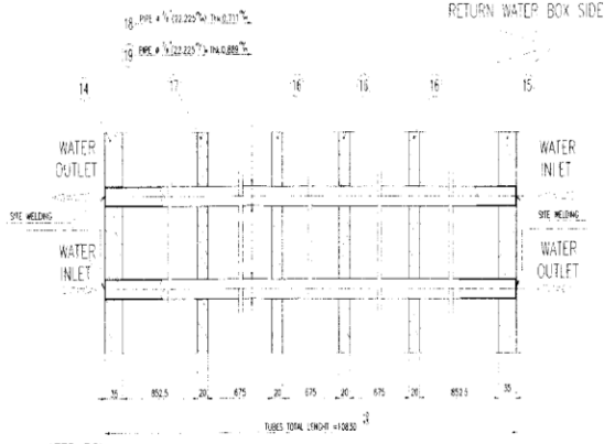
HEATING CONNECTIONS TUBE BUNDLE DETAIL FOR ROLLING AND WELDING DETAIL SEE RELEVANT SPECIFICATION
