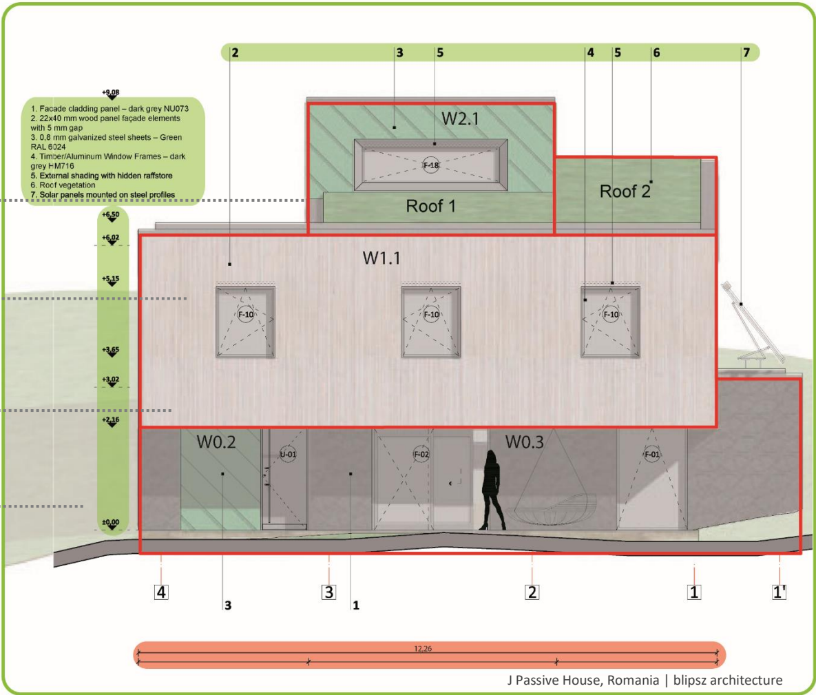
Graphic identification and external dimensions of the thermal envelope
