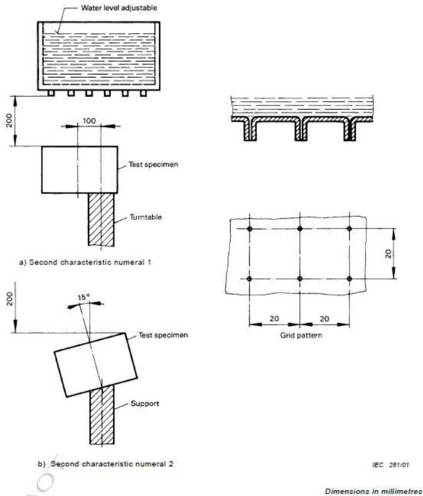
Figure 4 – (Figure 3 according to IEC 60529) Test device to verify protection against falling water drops - Drip Box for IPX1, IPX2
