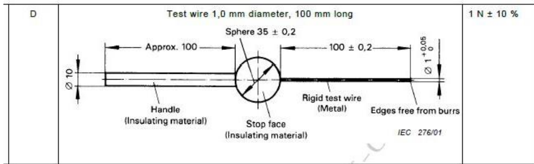
Figure 2 – Test equipment for IPXXD
