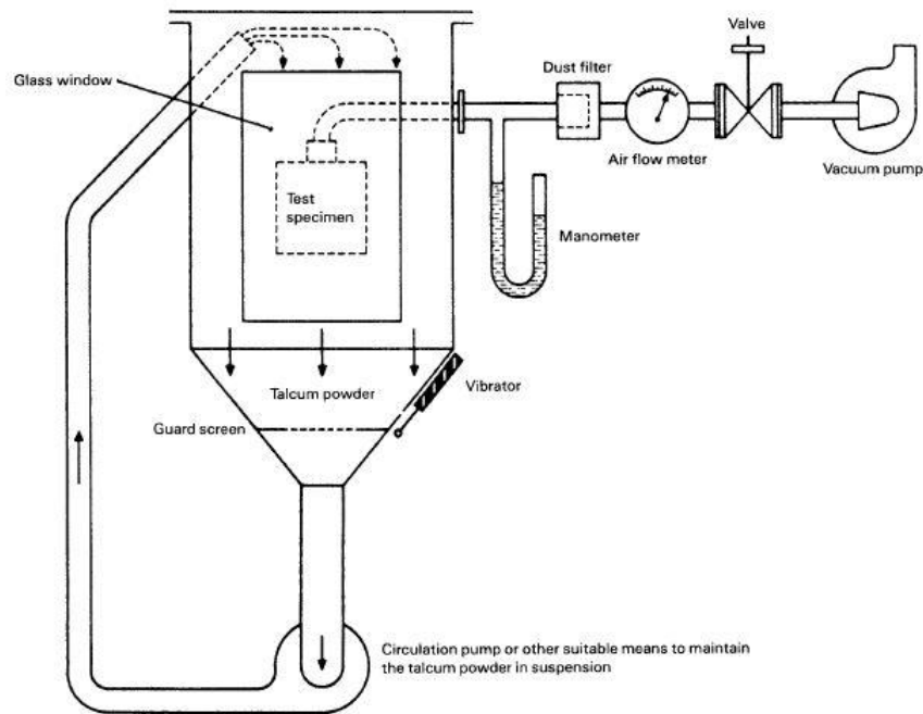
Figure 1 – Dust chamber with vacuum pump (figure 2 according to IEC 60529)
