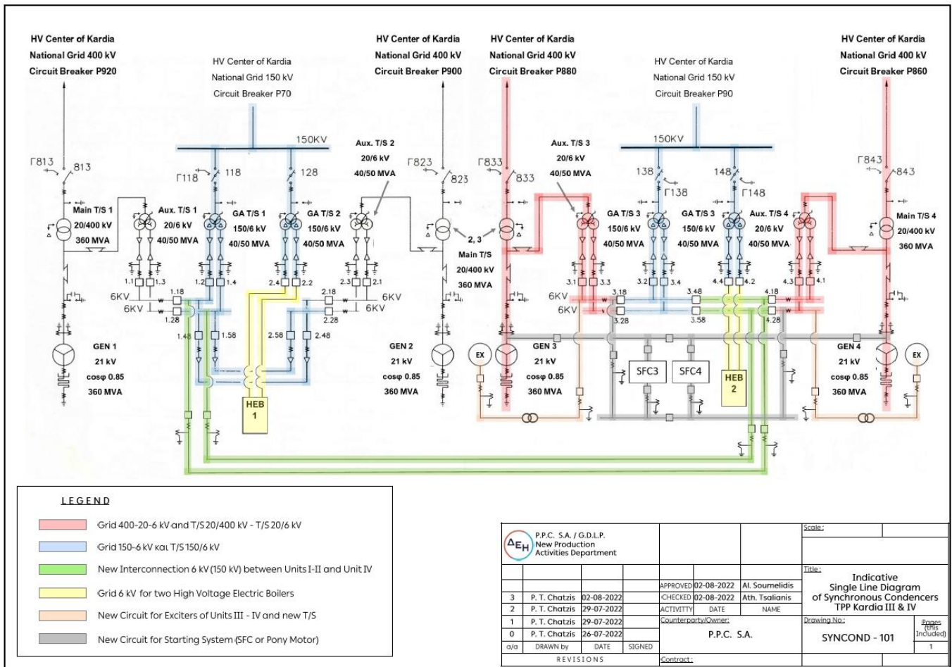
FIGURE 2: Indicative SLD of SFCs' installation
