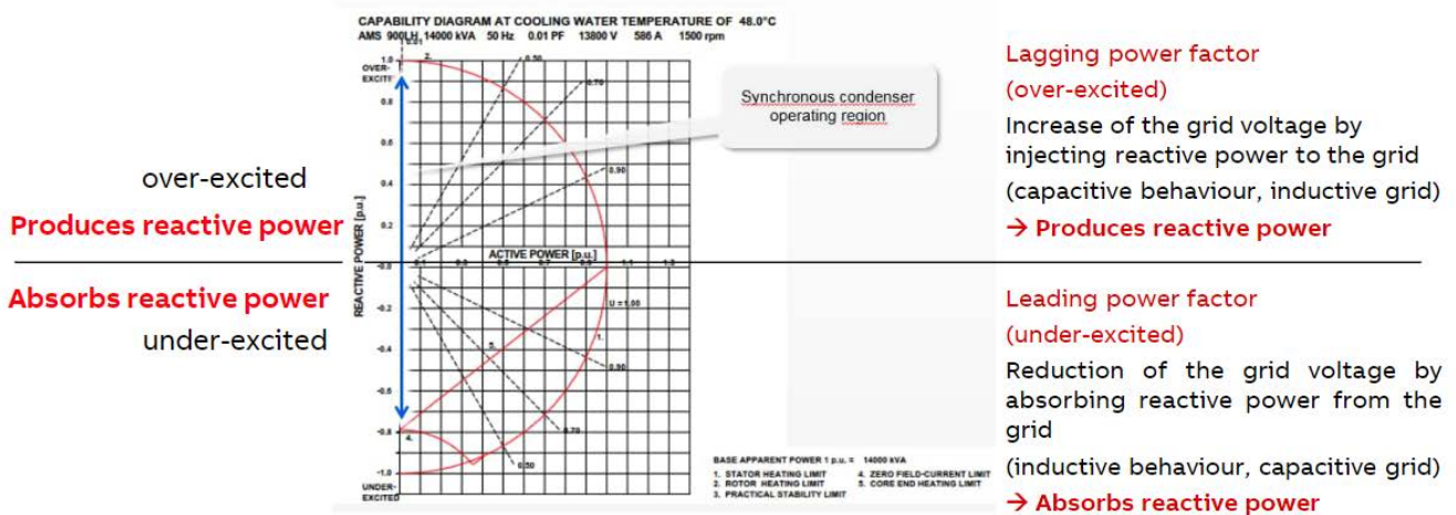
FIGURE 3: Generators capability curve
