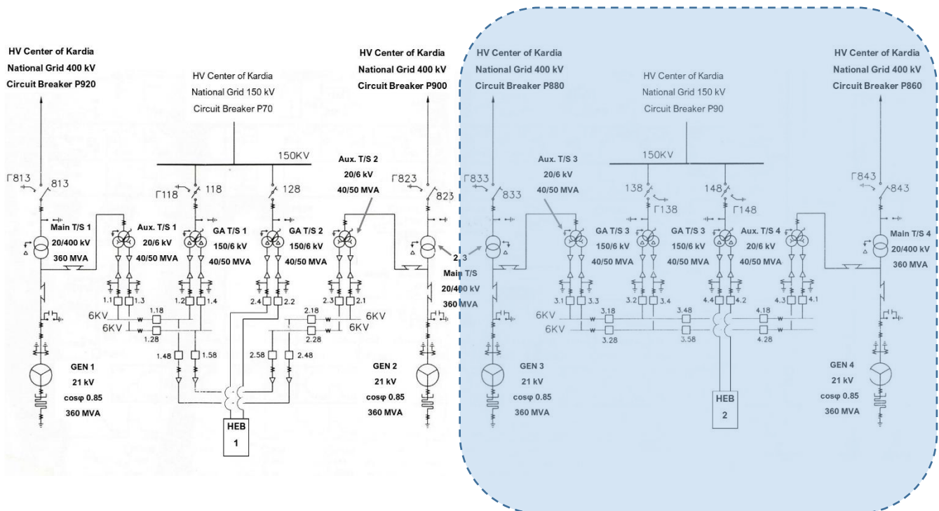
FIGURE 1: SLD of 400 & 150 kV grid of TPP-K
