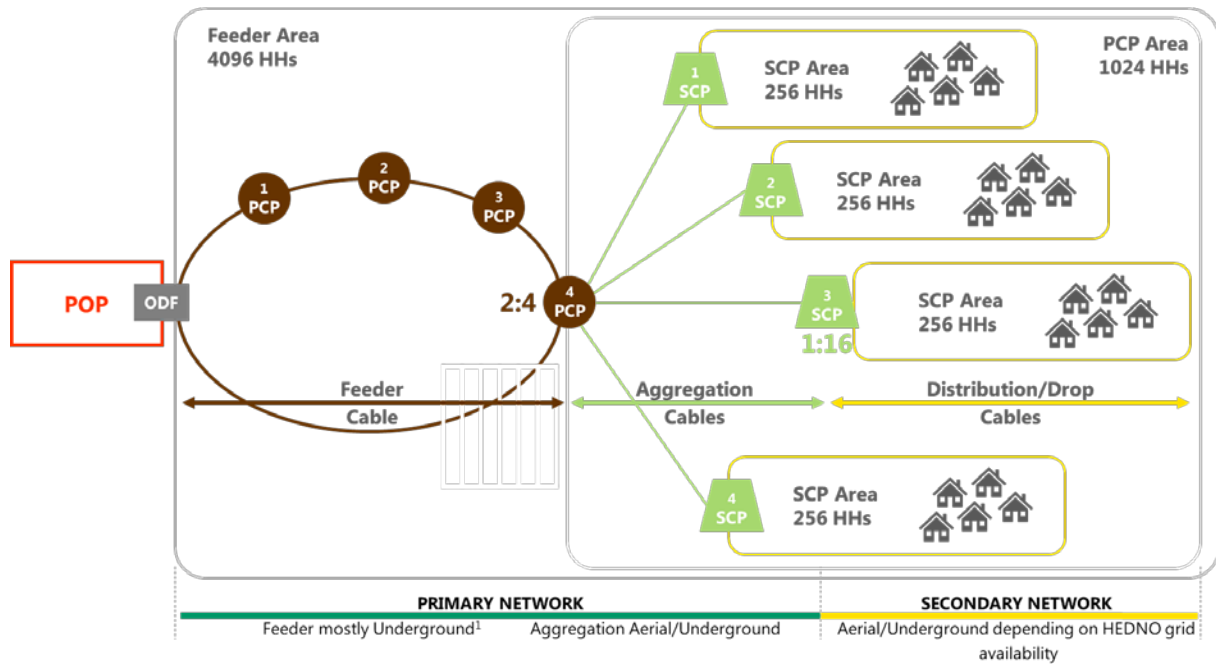
Figure 3 - Network Areas
