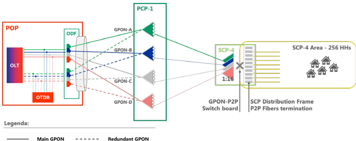
Figure 6 - PCP Area and SCPs
