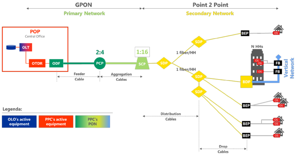
Figure 4 - Cables
