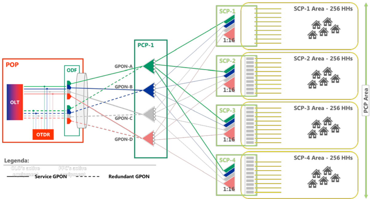
Figure 5 - PCP-2-SCP splicing schema
