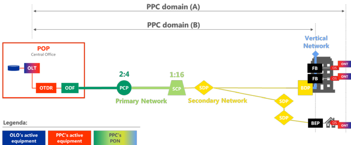
Figure 2 - PPC Domains
