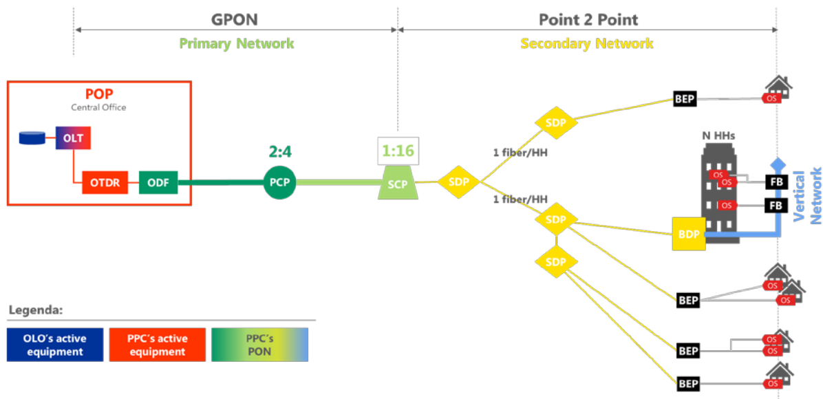
Figure 1 - Network Architecture
