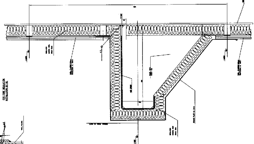
DETAIL 11 TANK WALL INSULATION
