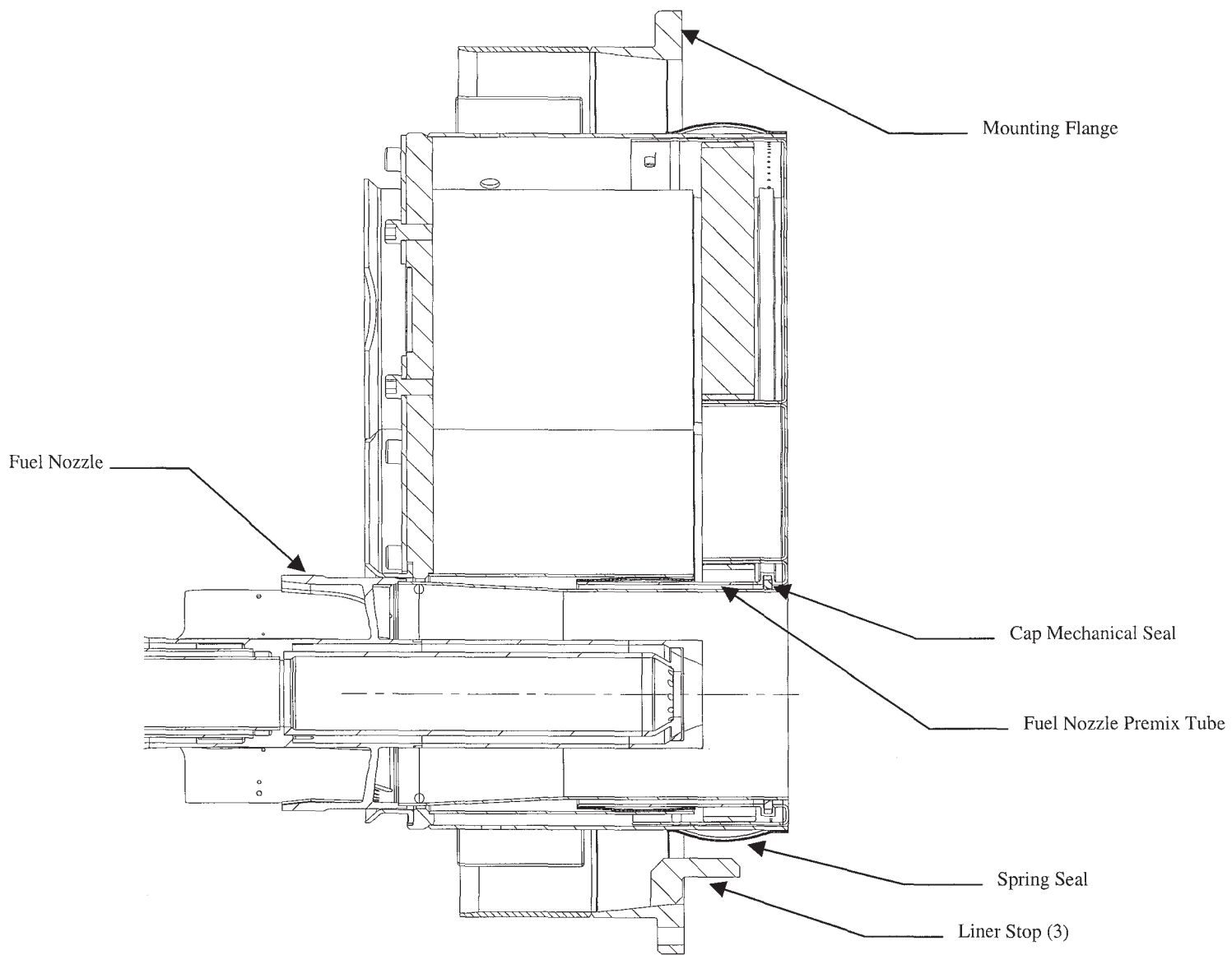
Figure CI-I.6. Cap Assembly with Fuel Nozzle
